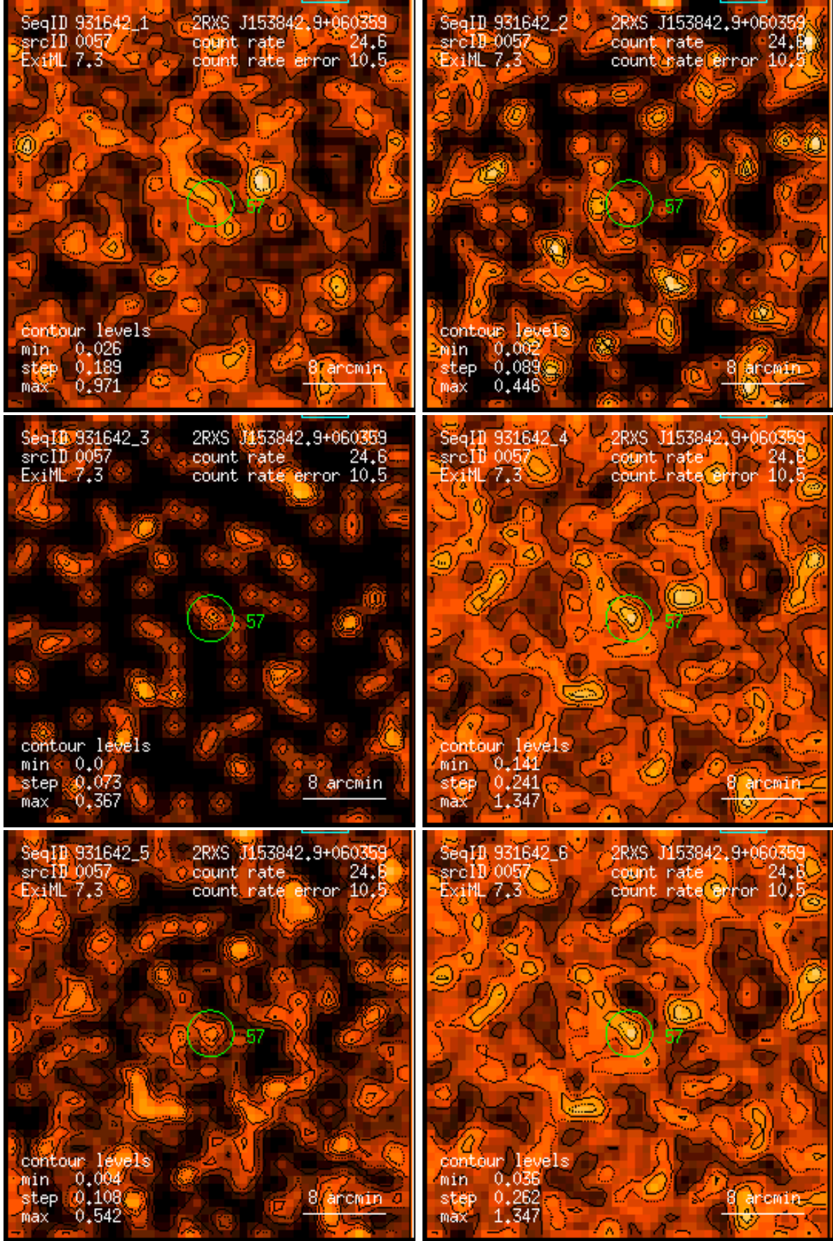
Figure 57: RASS 931642: detection 0057: band rate images, Gaussian filter: (1) PSPC channels 11 – 41, (2) 52 – 90, (3) 91 – 201, (4) 11 – 235, (5) 52 – 201, (6) 11 – 201. Broad band rates in counts/ks. Band rate contour levels in counts/ks/arcmin 2 .
