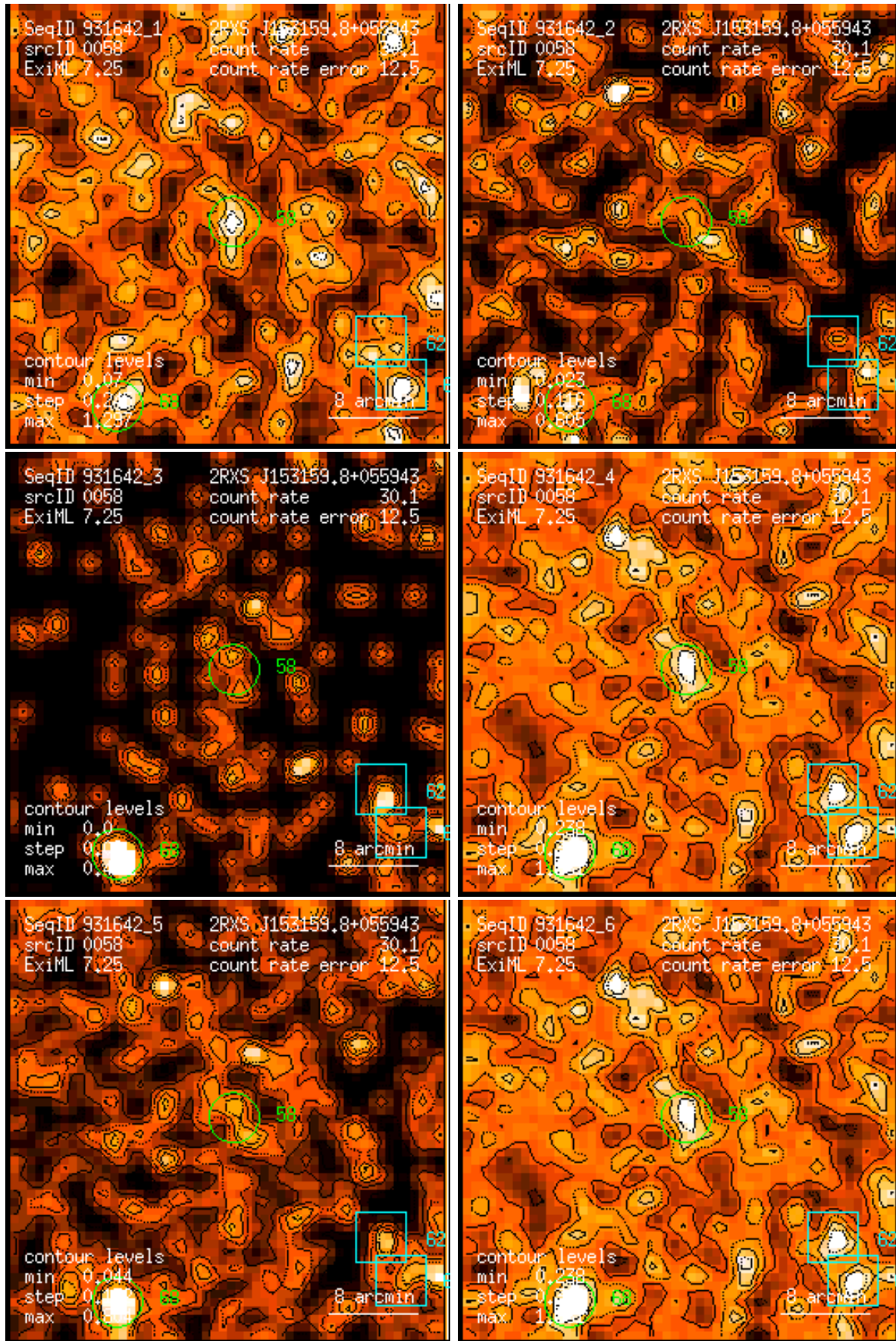
Figure 58: RASS 931642: detection 0058: band rate images, Gaussian filter: (1) PSPC channels 11 – 41, (2) 52 – 90, (3) 91 – 201, (4) 11 – 235, (5) 52 – 201, (6) 11 – 201. Broad band rates in counts/ks. Band rate contour levels in counts/ks/arcmin 2 .
