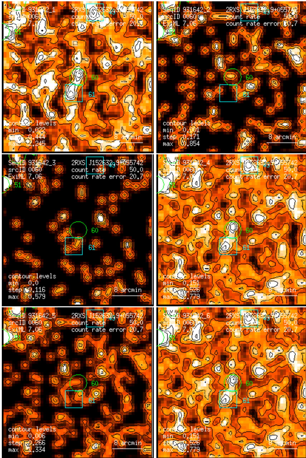
Figure 60: RASS 931642: detection 0060: band rate images, Gaussian filter: (1) PSPC channels 11 – 41, (2) 52 – 90, (3) 91 – 201, (4) 11 – 235, (5) 52 – 201, (6) 11 – 201. Broad band rates in counts/ks. Band rate contour levels in counts/ks/arcmin 2 .
