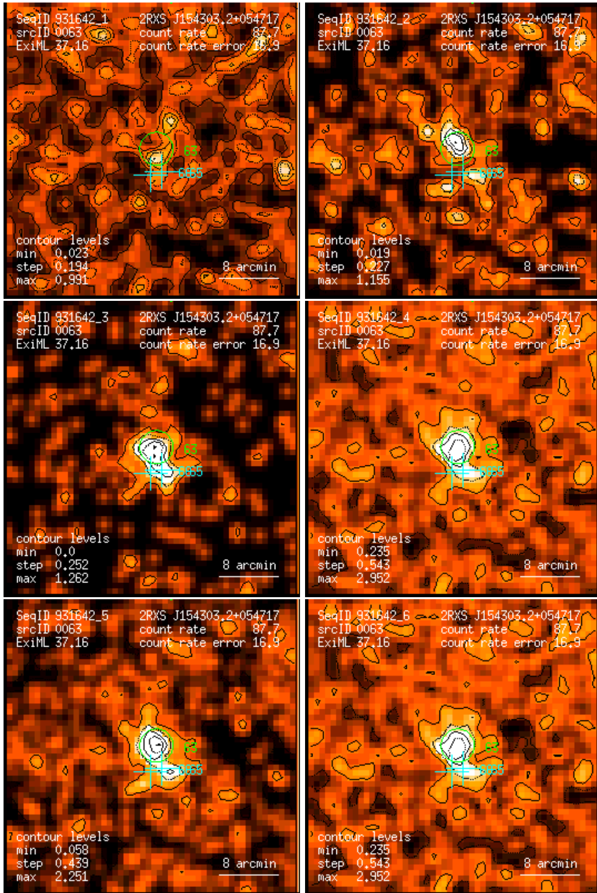
Figure 63: RASS 931642: detection 0063: band rate images, Gaussian filter: (1) PSPC channels 11 – 41, (2) 52 – 90, (3) 91 – 201, (4) 11 – 235, (5) 52 – 201, (6) 11 – 201. Broad band rates in counts/ks. Band rate contour levels in counts/ks/arcmin 2 .
