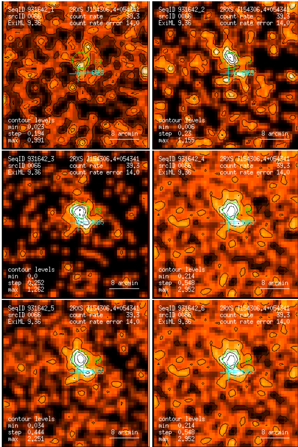
Figure 66: RASS 931642: detection 0066: band rate images, Gaussian filter: (1) PSPC channels 11 – 41, (2) 52 – 90, (3) 91 – 201, (4) 11 – 235, (5) 52 – 201, (6) 11 – 201. Broad band rates in counts/ks. Band rate contour levels in counts/ks/arcmin 2 .
