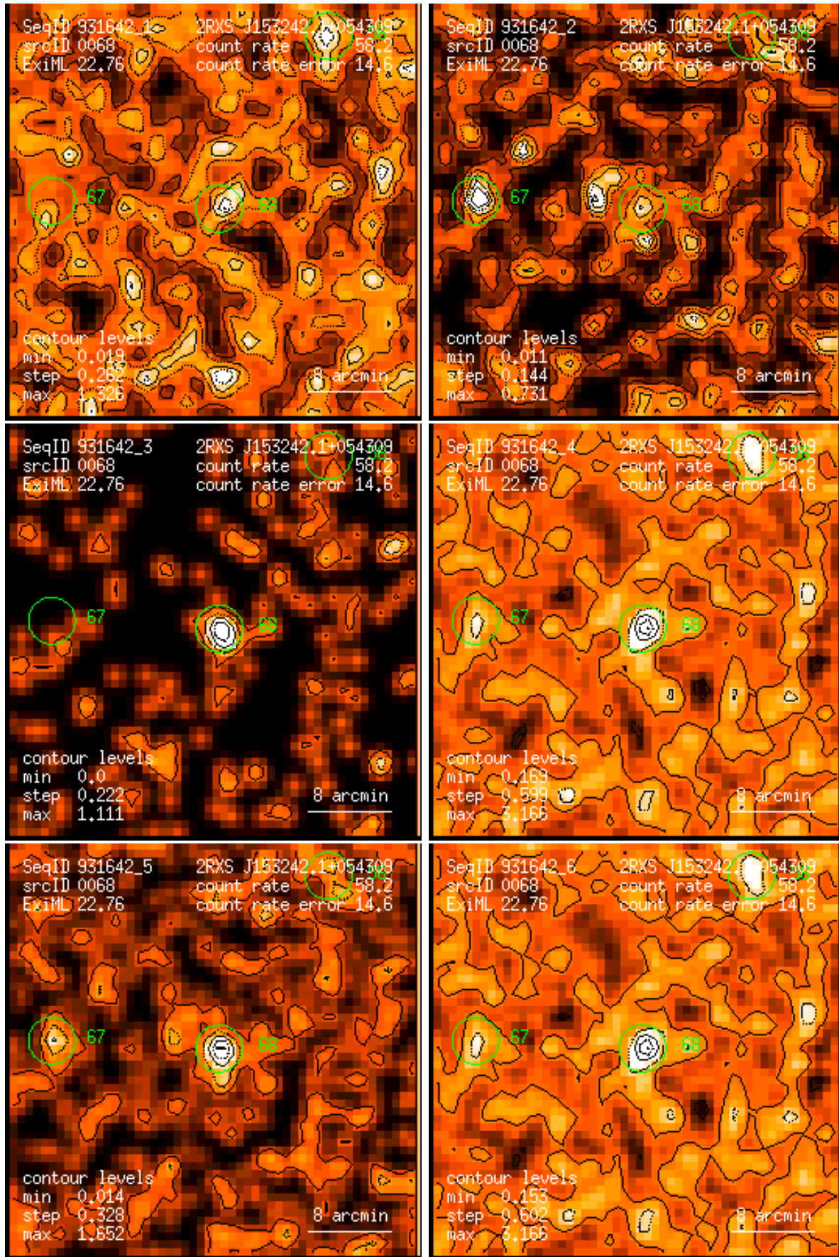
Figure 68: RASS 931642: detection 0068: band rate images, Gaussian filter: (1) PSPC channels 11 – 41, (2) 52 – 90, (3) 91 – 201, (4) 11 – 235, (5) 52 – 201, (6) 11 – 201. Broad band rates in counts/ks. Band rate contour levels in counts/ks/arcmin 2 .
