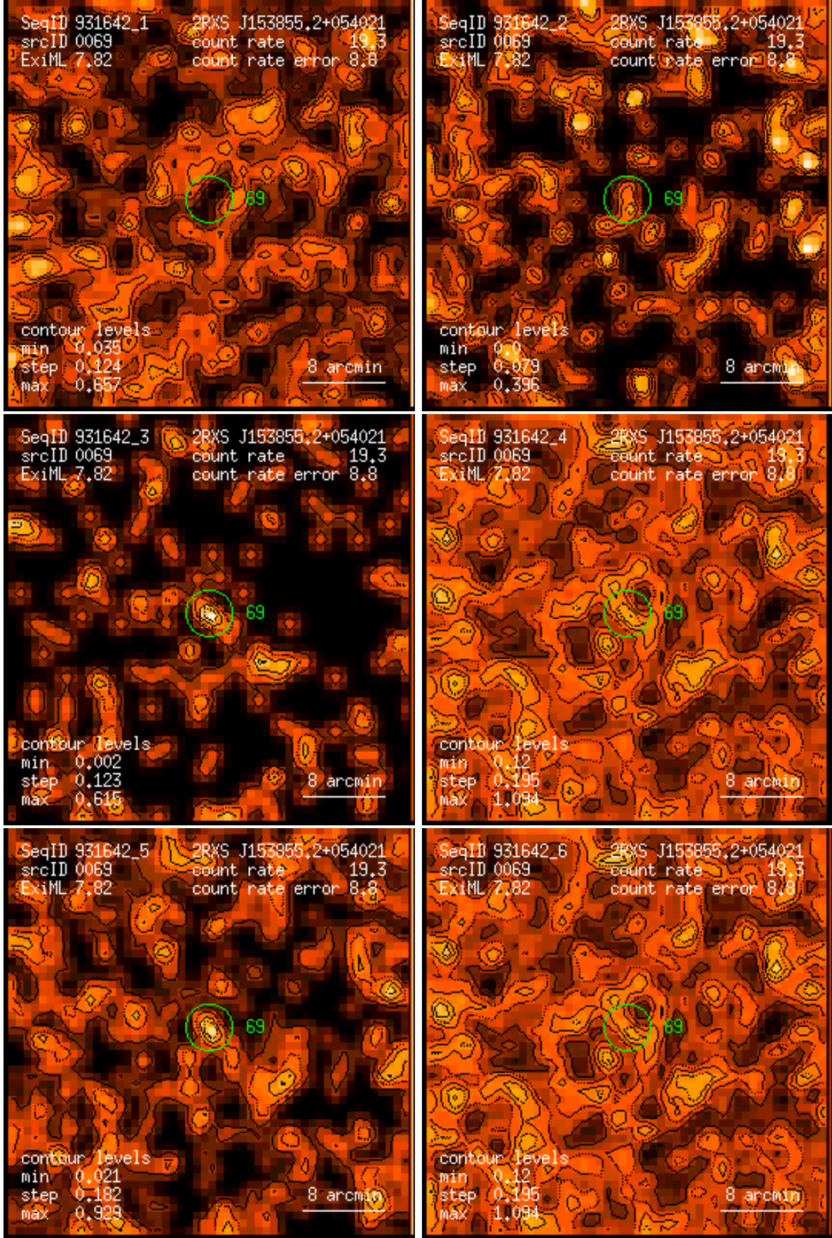
Figure 69: RASS 931642: detection 0069: band rate images, Gaussian filter: (1) PSPC channels 11 – 41, (2) 52 – 90, (3) 91 – 201, (4) 11 – 235, (5) 52 – 201, (6) 11 – 201. Broad band rates in counts/ks. Band rate contour levels in counts/ks/arcmin 2 .
