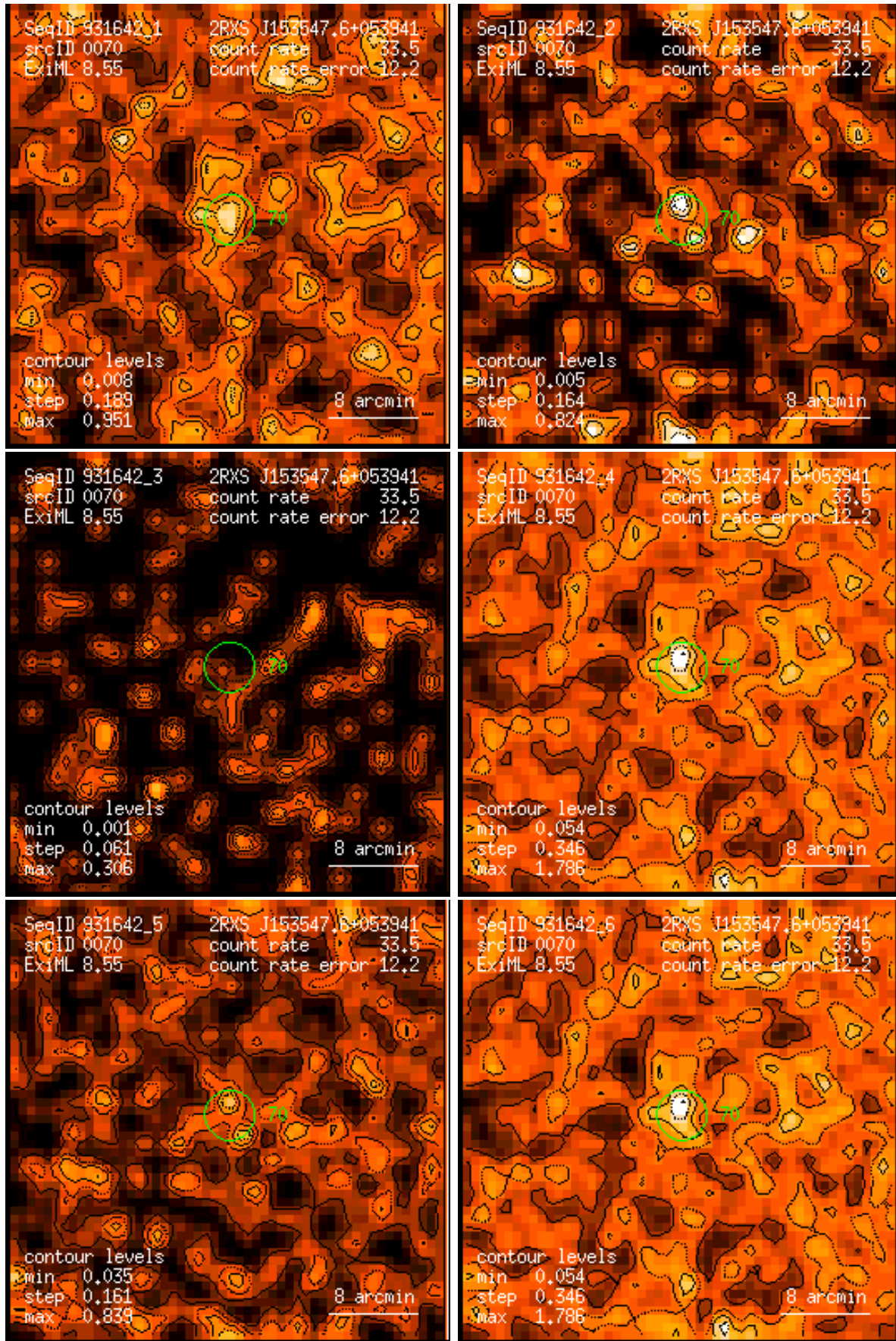
Figure 70: RASS 931642: detection 0070: band rate images, Gaussian filter: (1) PSPC channels 11 – 41, (2) 52 – 90, (3) 91 – 201, (4) 11 – 235, (5) 52 – 201, (6) 11 – 201. Broad band rates in counts/ks. Band rate contour levels in counts/ks/arcmin 2 .
