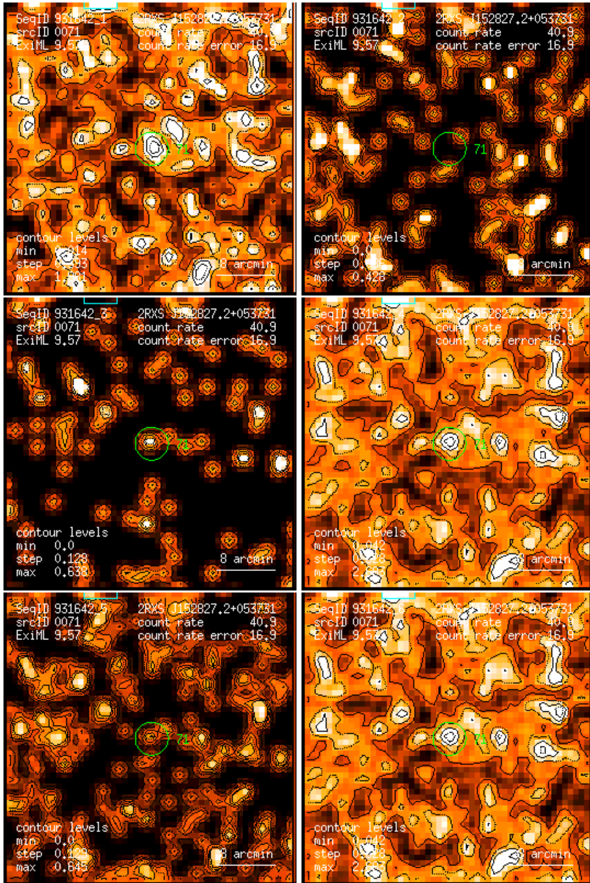
Figure 71: RASS 931642: detection 0071: band rate images, Gaussian filter: (1) PSPC channels 11 – 41, (2) 52 – 90, (3) 91 – 201, (4) 11 – 235, (5) 52 – 201, (6) 11 – 201. Broad band rates in counts/ks. Band rate contour levels in counts/ks/arcmin 2 .
