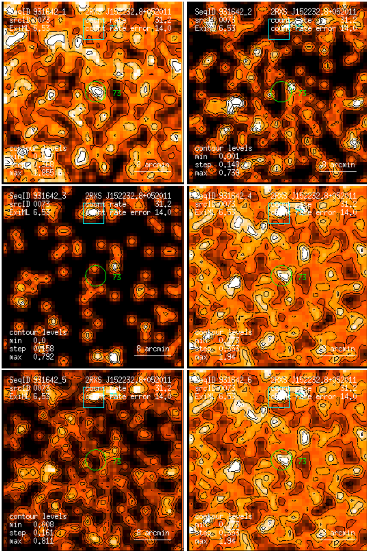
Figure 73: RASS 931642: detection 0073: band rate images, Gaussian filter: (1) PSPC channels 11 – 41, (2) 52 – 90, (3) 91 – 201, (4) 11 – 235, (5) 52 – 201, (6) 11 – 201. Broad band rates in counts/ks. Band rate contour levels in counts/ks/arcmin 2 .
