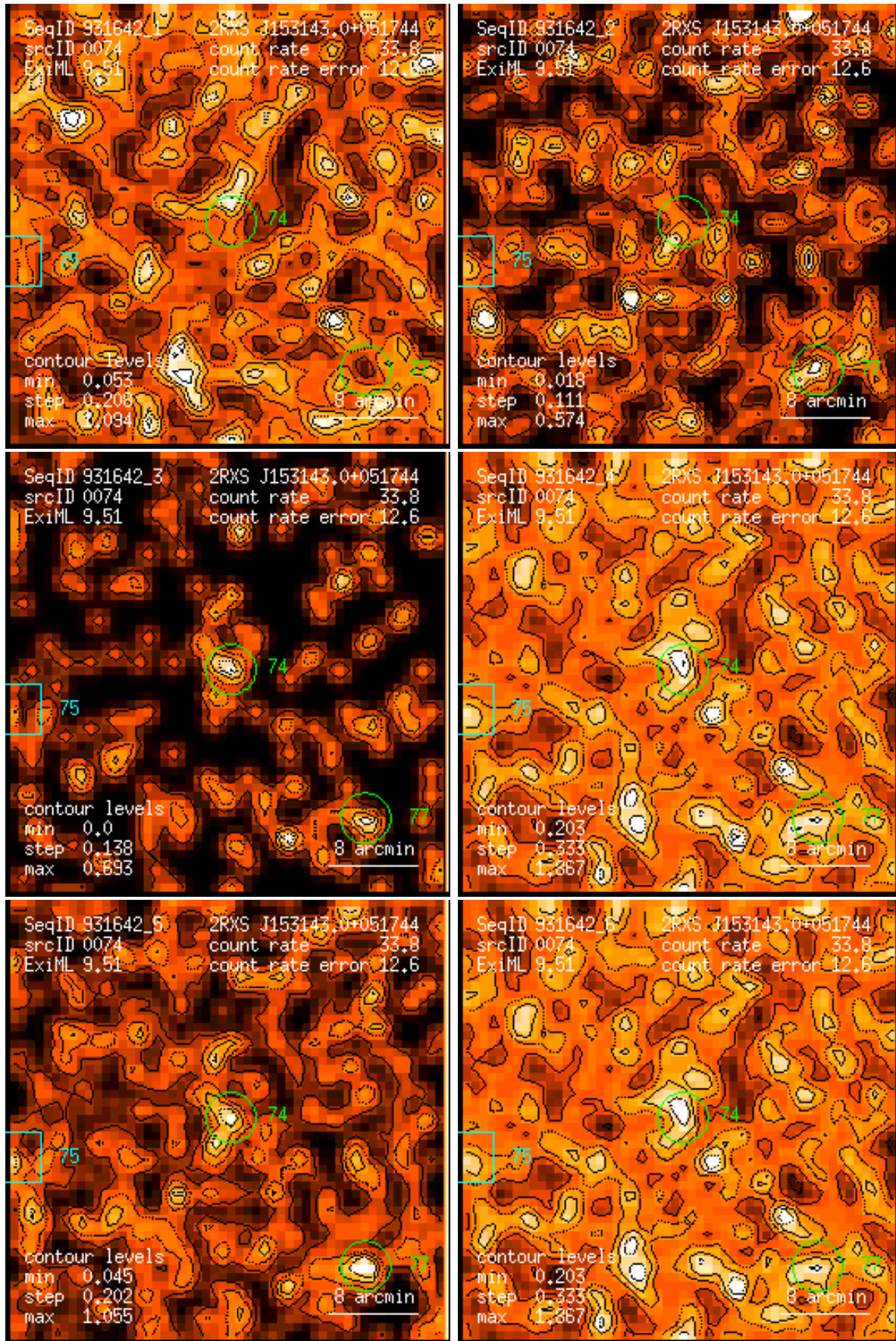
Figure 74: RASS 931642: detection 0074: band rate images, Gaussian filter: (1) PSPC channels 11 – 41, (2) 52 – 90, (3) 91 – 201, (4) 11 – 235, (5) 52 – 201, (6) 11 – 201. Broad band rates in counts/ks. Band rate contour levels in counts/ks/arcmin 2 .
