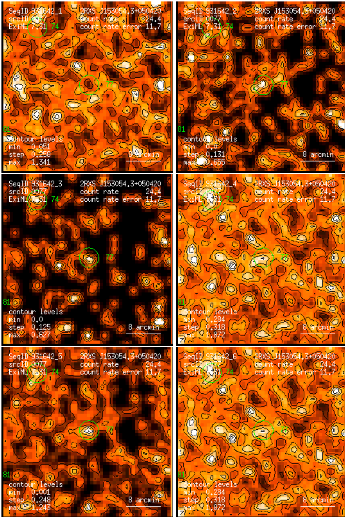
Figure 77: RASS 931642: detection 0077: band rate images, Gaussian filter: (1) PSPC channels 11 – 41, (2) 52 – 90, (3) 91 – 201, (4) 11 – 235, (5) 52 – 201, (6) 11 – 201. Broad band rates in counts/ks. Band rate contour levels in counts/ks/arcmin 2 .
