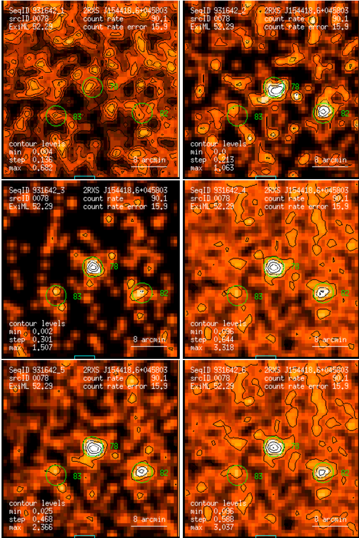
Figure 78: RASS 931642: detection 0078: band rate images, Gaussian filter: (1) PSPC channels 11 – 41, (2) 52 – 90, (3) 91 – 201, (4) 11 – 235, (5) 52 – 201, (6) 11 – 201. Broad band rates in counts/ks. Band rate contour levels in counts/ks/arcmin 2 .
