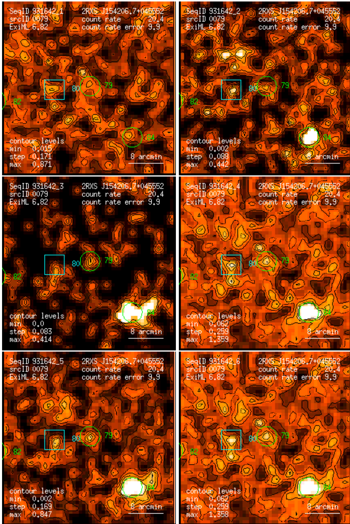
Figure 79: RASS 931642: detection 0079: band rate images, Gaussian filter: (1) PSPC channels 11 – 41, (2) 52 – 90, (3) 91 – 201, (4) 11 – 235, (5) 52 – 201, (6) 11 – 201. Broad band rates in counts/ks. Band rate contour levels in counts/ks/arcmin 2 .
