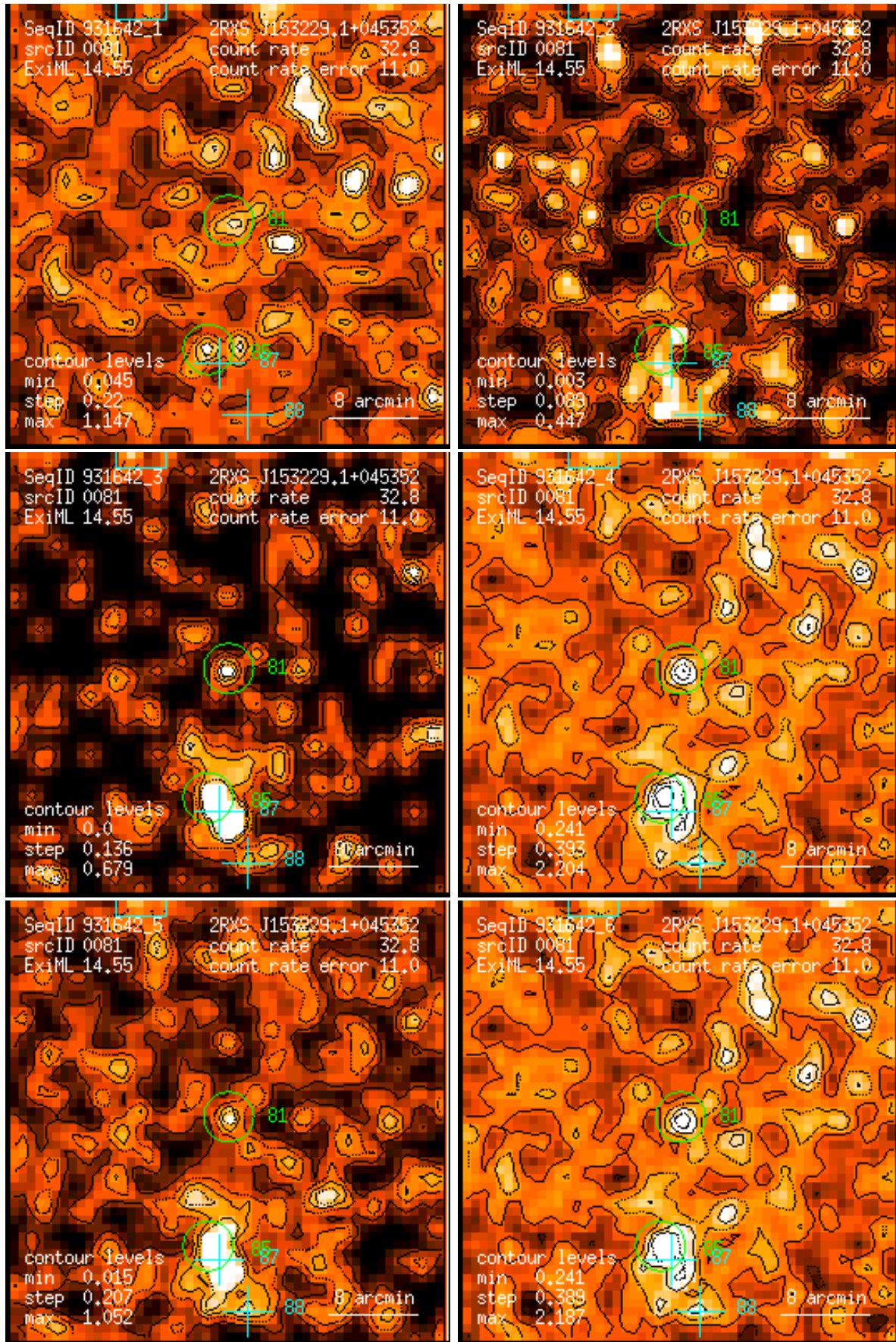
Figure 81: RASS 931642: detection 0081: band rate images, Gaussian filter: (1) PSPC channels 11 – 41, (2) 52 – 90, (3) 91 – 201, (4) 11 – 235, (5) 52 – 201, (6) 11 – 201. Broad band rates in counts/ks. Band rate contour levels in counts/ks/arcmin 2 .
