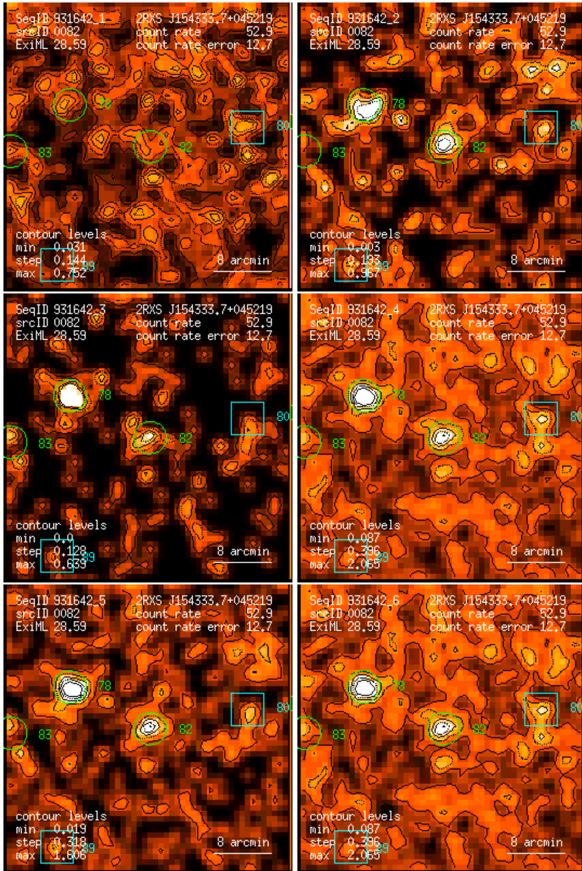
Figure 82: RASS 931642: detection 0082: band rate images, Gaussian filter: (1) PSPC channels 11 – 41, (2) 52 – 90, (3) 91 – 201, (4) 11 – 235, (5) 52 – 201, (6) 11 – 201. Broad band rates in counts/ks. Band rate contour levels in counts/ks/arcmin 2 .
