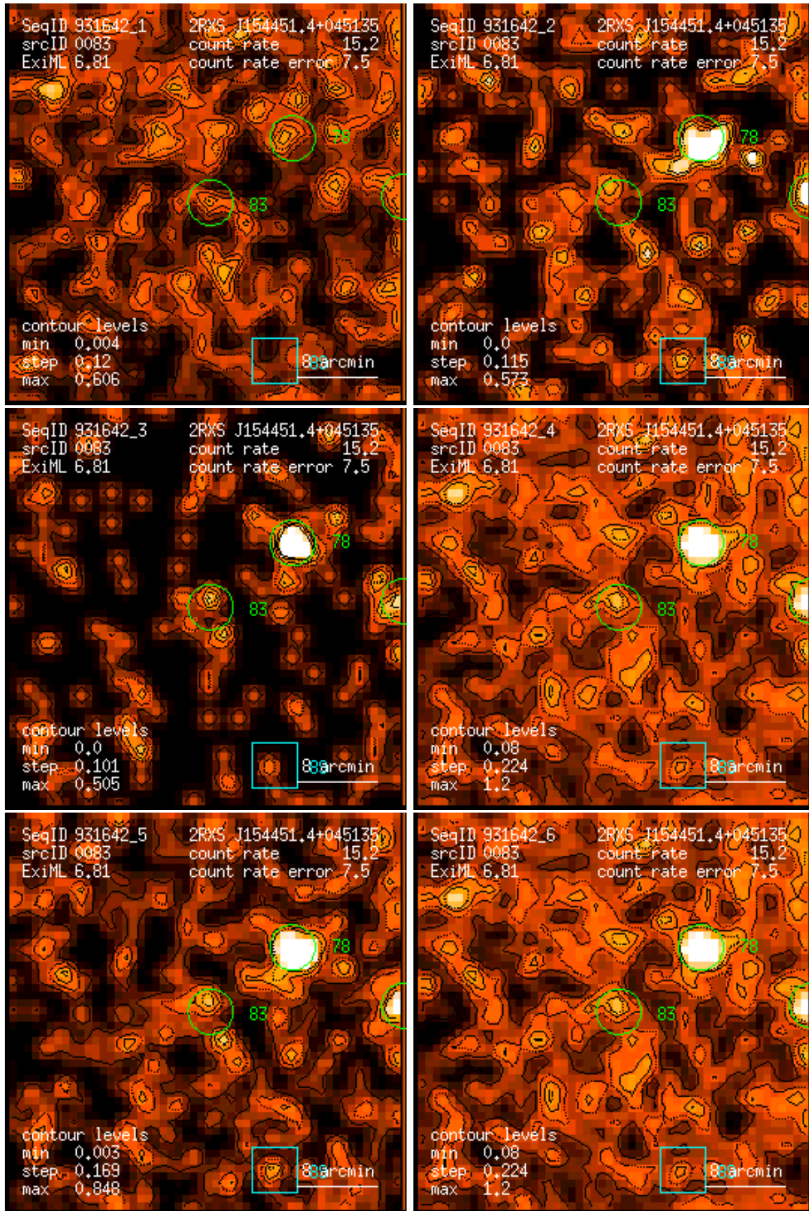
Figure 83: RASS 931642: detection 0083: band rate images, Gaussian filter: (1) PSPC channels 11 – 41, (2) 52 – 90, (3) 91 – 201, (4) 11 – 235, (5) 52 – 201, (6) 11 – 201. Broad band rates in counts/ks. Band rate contour levels in counts/ks/arcmin 2 .
