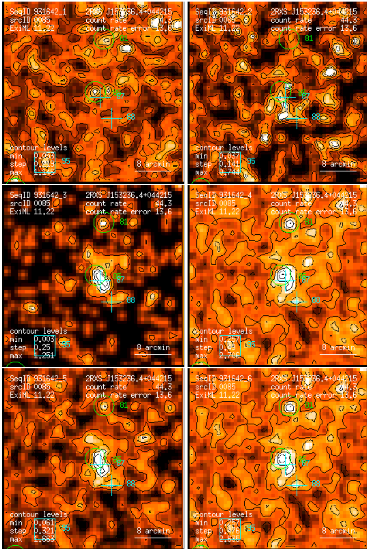
Figure 85: RASS 931642: detection 0085: band rate images, Gaussian filter: (1) PSPC channels 11 – 41, (2) 52 – 90, (3) 91 – 201, (4) 11 – 235, (5) 52 – 201, (6) 11 – 201. Broad band rates in counts/ks. Band rate contour levels in counts/ks/arcmin 2 .
