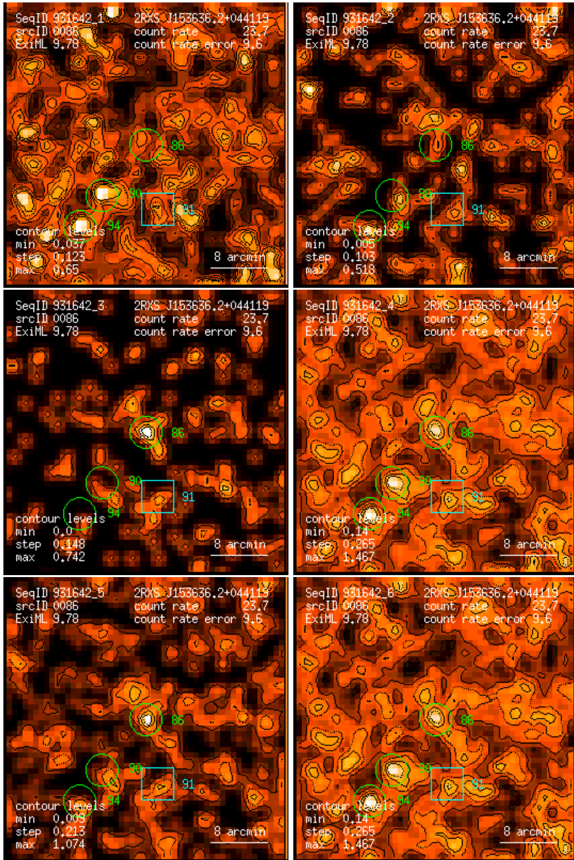
Figure 86: RASS 931642: detection 0086: band rate images, Gaussian filter: (1) PSPC channels 11 – 41, (2) 52 – 90, (3) 91 – 201, (4) 11 – 235, (5) 52 – 201, (6) 11 – 201. Broad band rates in counts/ks. Band rate contour levels in counts/ks/arcmin 2 .
