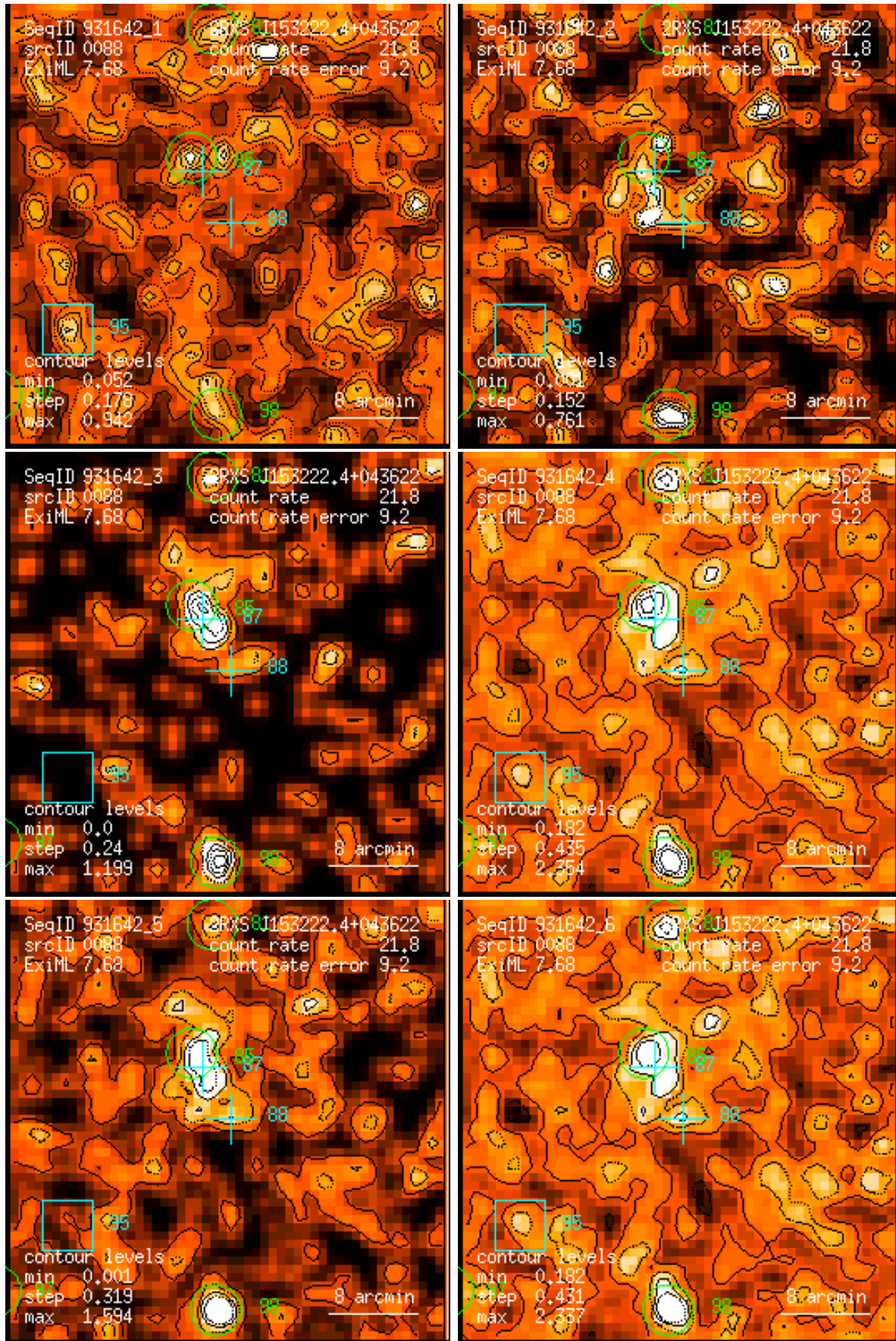
Figure 88: RASS 931642: detection 0088: band rate images, Gaussian filter: (1) PSPC channels 11 – 41, (2) 52 – 90, (3) 91 – 201, (4) 11 – 235, (5) 52 – 201, (6) 11 – 201. Broad band rates in counts/ks. Band rate contour levels in counts/ks/arcmin 2 .
