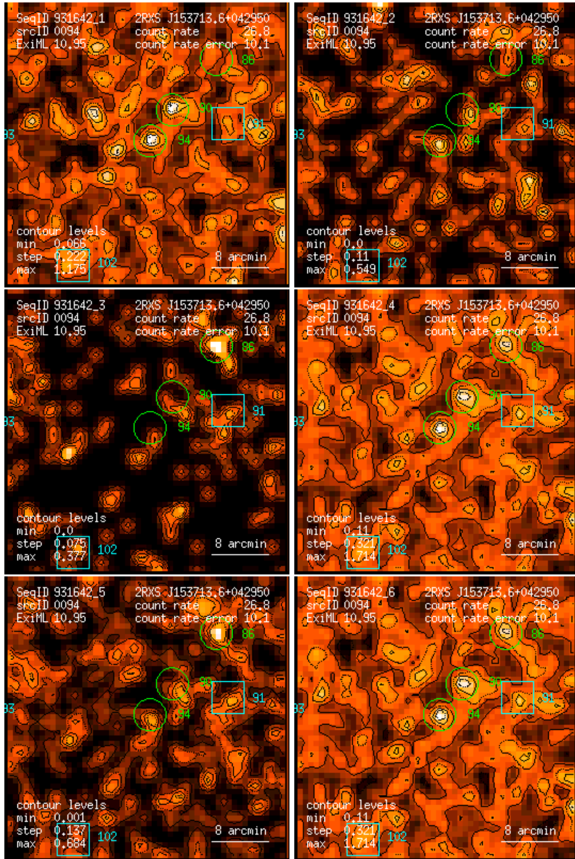
Figure 94: RASS 931642: detection 0094: band rate images, Gaussian filter: (1) PSPC channels 11 – 41, (2) 52 – 90, (3) 91 – 201, (4) 11 – 235, (5) 52 – 201, (6) 11 – 201. Broad band rates in counts/ks. Band rate contour levels in counts/ks/arcmin 2 .
