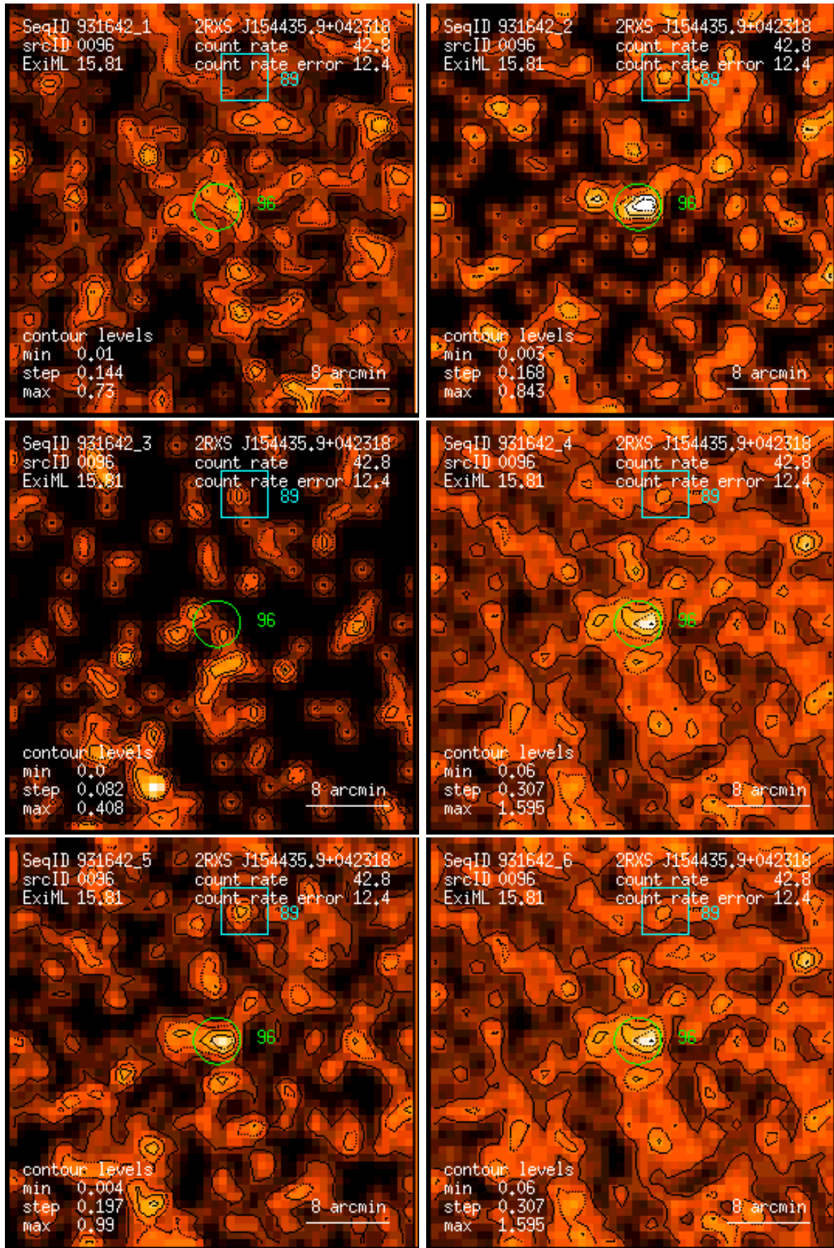
Figure 96: RASS 931642: detection 0096: band rate images, Gaussian filter: (1) PSPC channels 11 – 41, (2) 52 – 90, (3) 91 – 201, (4) 11 – 235, (5) 52 – 201, (6) 11 – 201. Broad band rates in counts/ks. Band rate contour levels in counts/ks/arcmin 2 .
