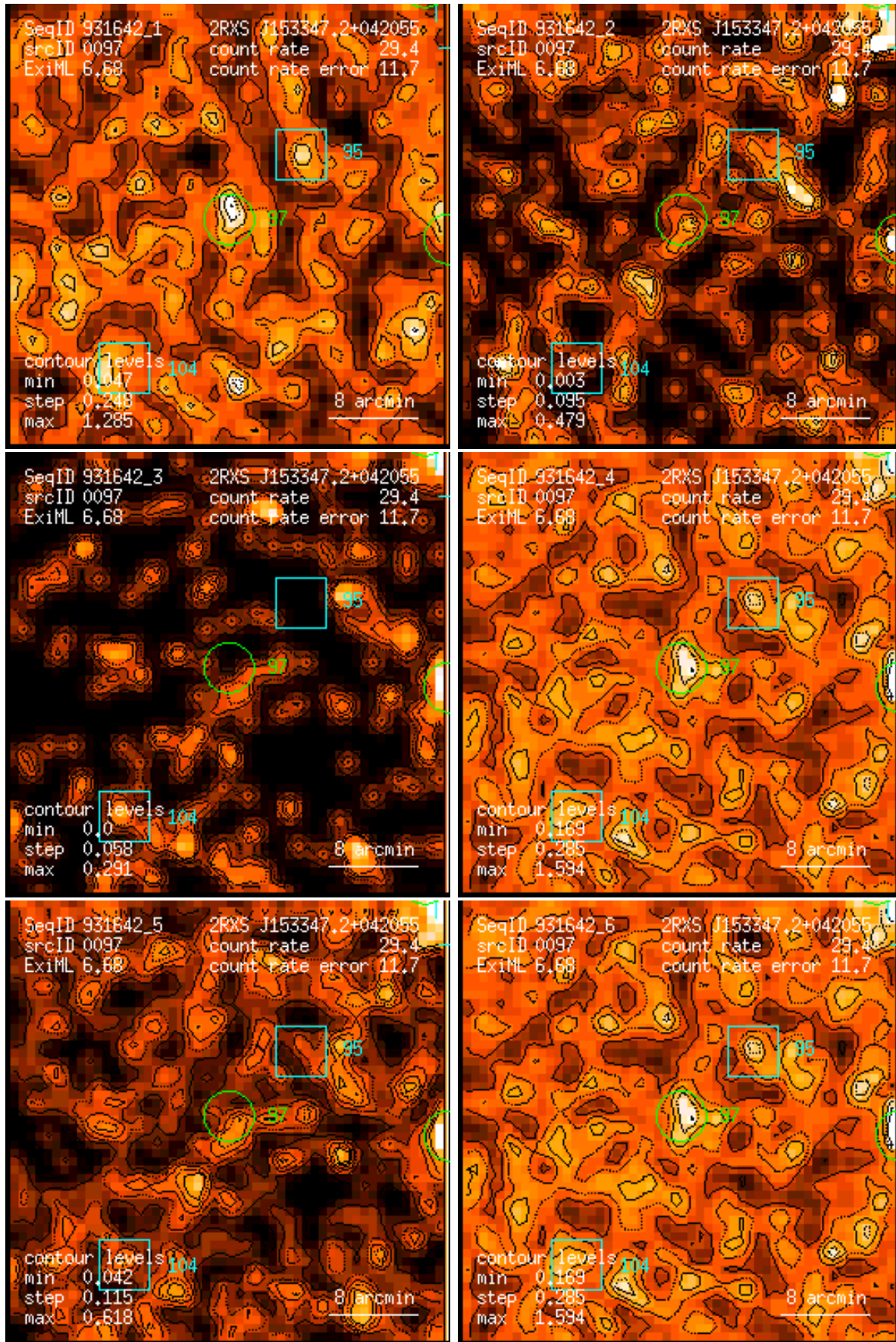
Figure 97: RASS 931642: detection 0097: band rate images, Gaussian filter: (1) PSPC channels 11 – 41, (2) 52 – 90, (3) 91 – 201, (4) 11 – 235, (5) 52 – 201, (6) 11 – 201. Broad band rates in counts/ks. Band rate contour levels in counts/ks/arcmin 2 .
