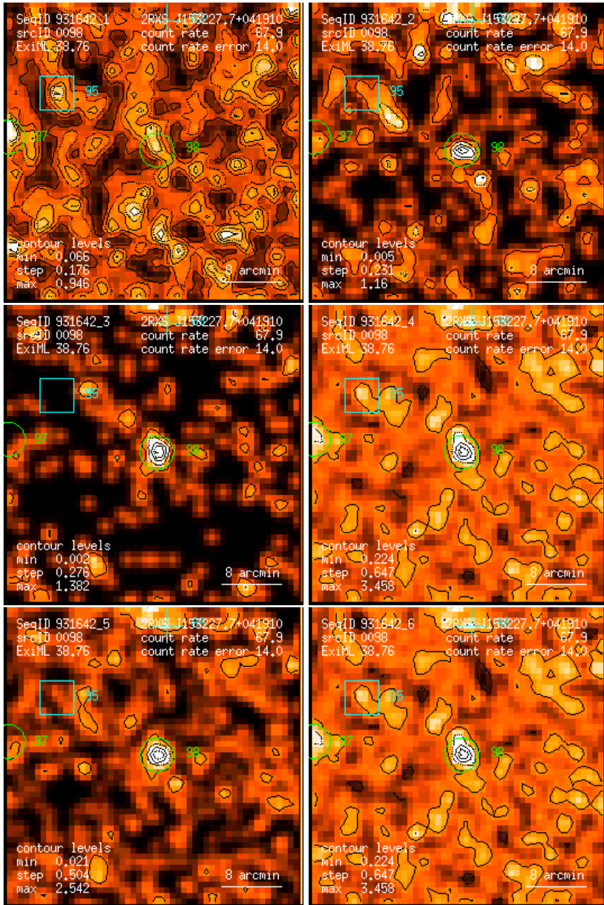
Figure 98: RASS 931642: detection 0098: band rate images, Gaussian filter: (1) PSPC channels 11 – 41, (2) 52 – 90, (3) 91 – 201, (4) 11 – 235, (5) 52 – 201, (6) 11 – 201. Broad band rates in counts/ks. Band rate contour levels in counts/ks/arcmin 2 .
