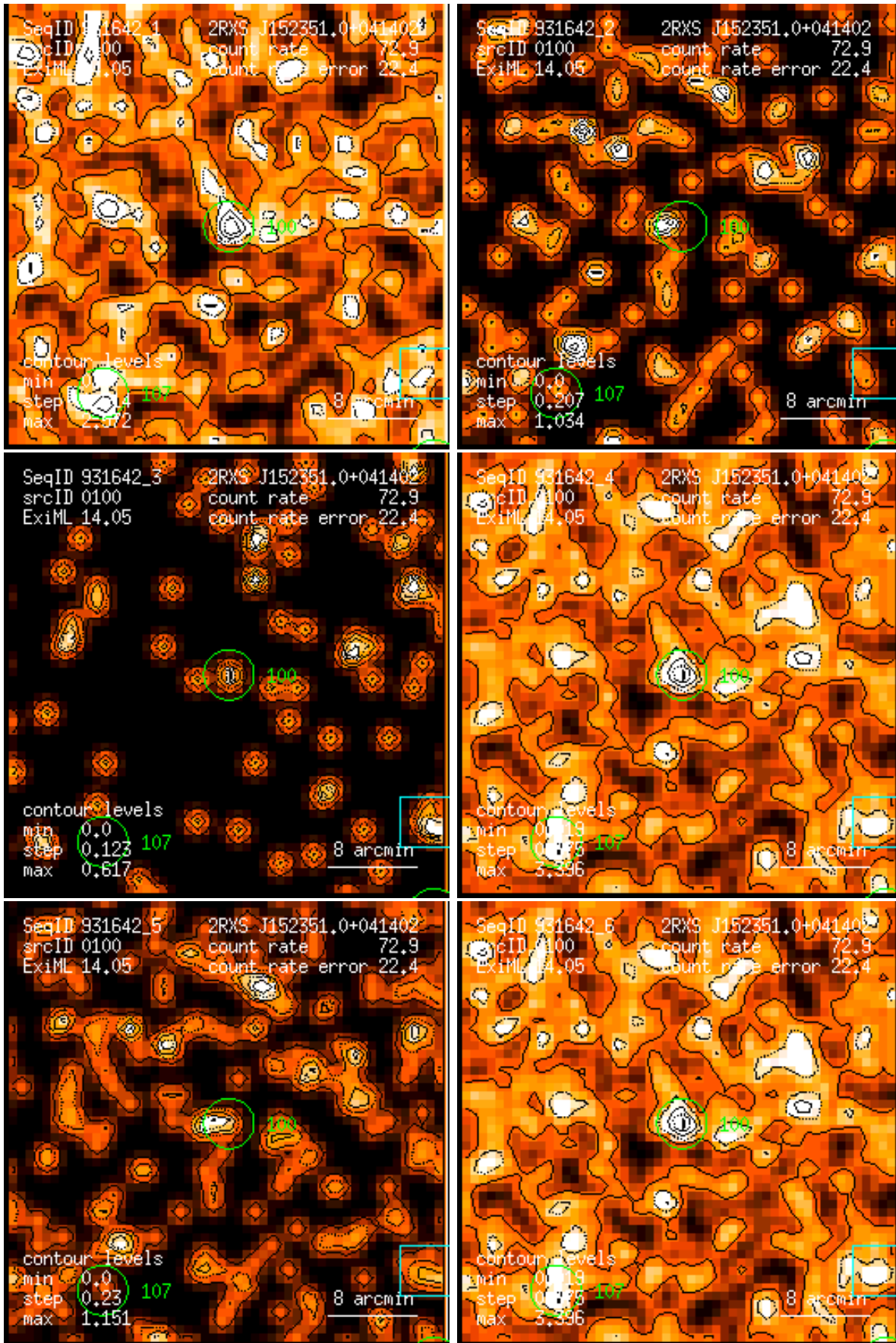
Figure 100: RASS 931642: detection 0100: band rate images, Gaussian filter: (1) PSPC channels 11 – 41, (2) 52 – 90, (3) 91 – 201, (4) 11 – 235, (5) 52 – 201, (6) 11 – 201. Broad band rates in counts/ks. Band rate contour levels in counts/ks/arcmin 2 .
