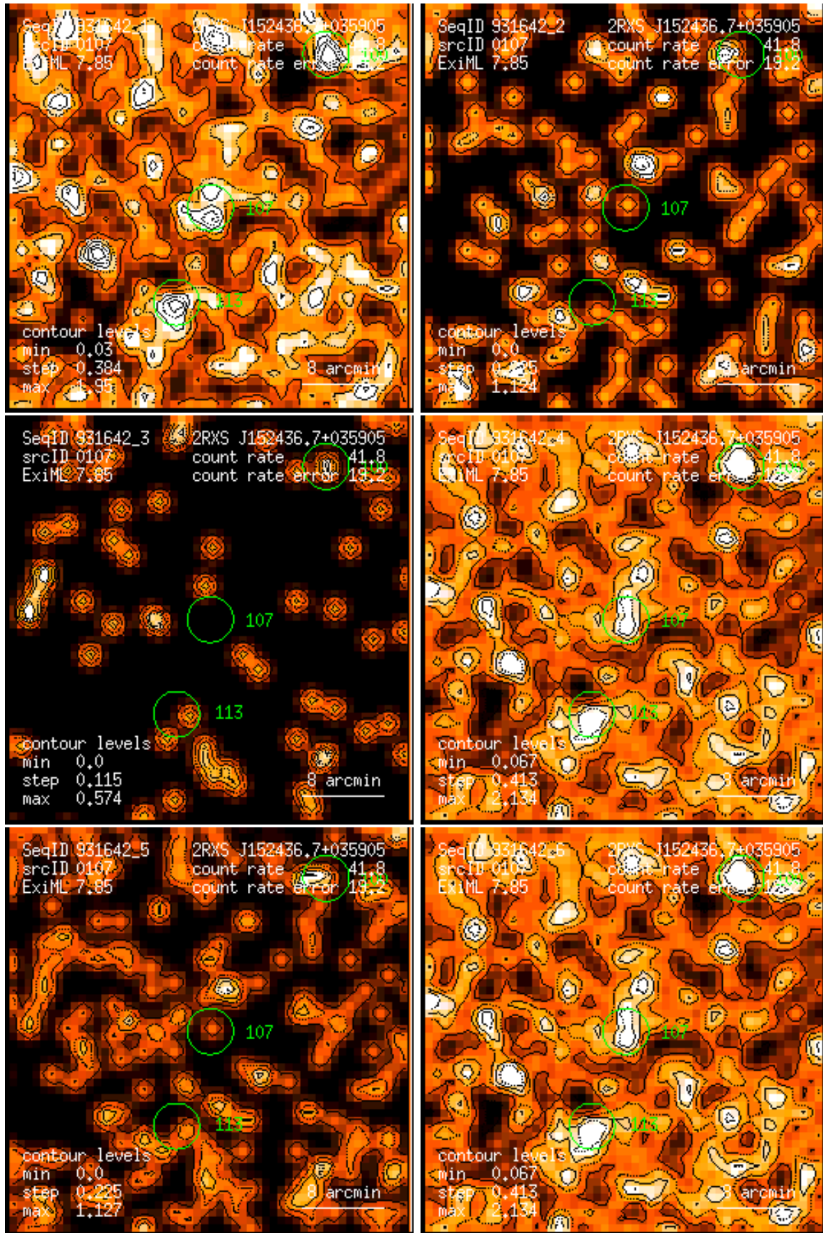
Figure 107: RASS 931642: detection 0107: band rate images, Gaussian filter: (1) PSPC channels 11 – 41, (2) 52 – 90, (3) 91 – 201, (4) 11 – 235, (5) 52 – 201, (6) 11 – 201. Broad band rates in counts/ks. Band rate contour levels in counts/ks/arcmin 2 .
