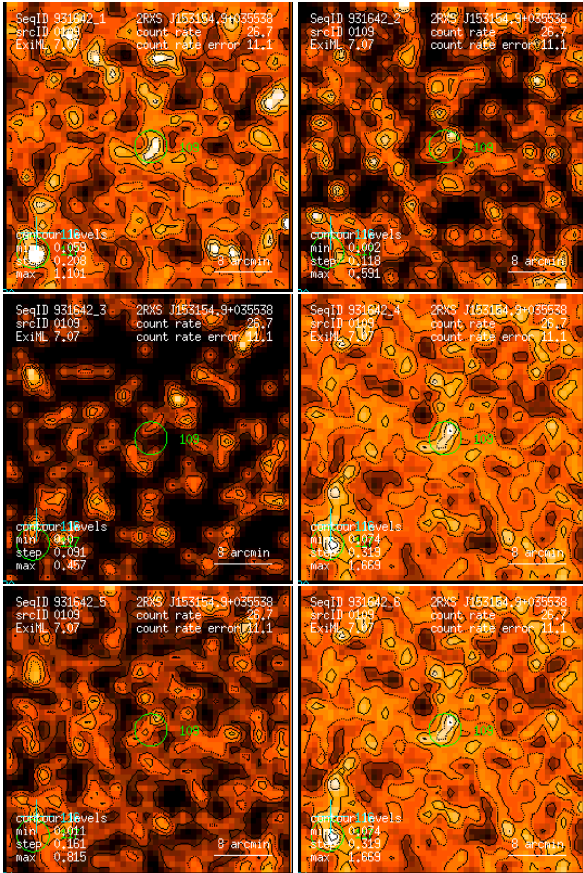
Figure 109: RASS 931642: detection 0109: band rate images, Gaussian filter: (1) PSPC channels 11 – 41, (2) 52 – 90, (3) 91 – 201, (4) 11 – 235, (5) 52 – 201, (6) 11 – 201. Broad band rates in counts/ks. Band rate contour levels in counts/ks/arcmin 2 .
