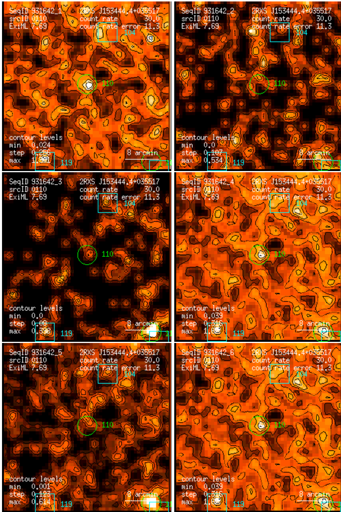
Figure 110: RASS 931642: detection 0110: band rate images, Gaussian filter: (1) PSPC channels 11 – 41, (2) 52 – 90, (3) 91 – 201, (4) 11 – 235, (5) 52 – 201, (6) 11 – 201. Broad band rates in counts/ks. Band rate contour levels in counts/ks/arcmin 2 .
