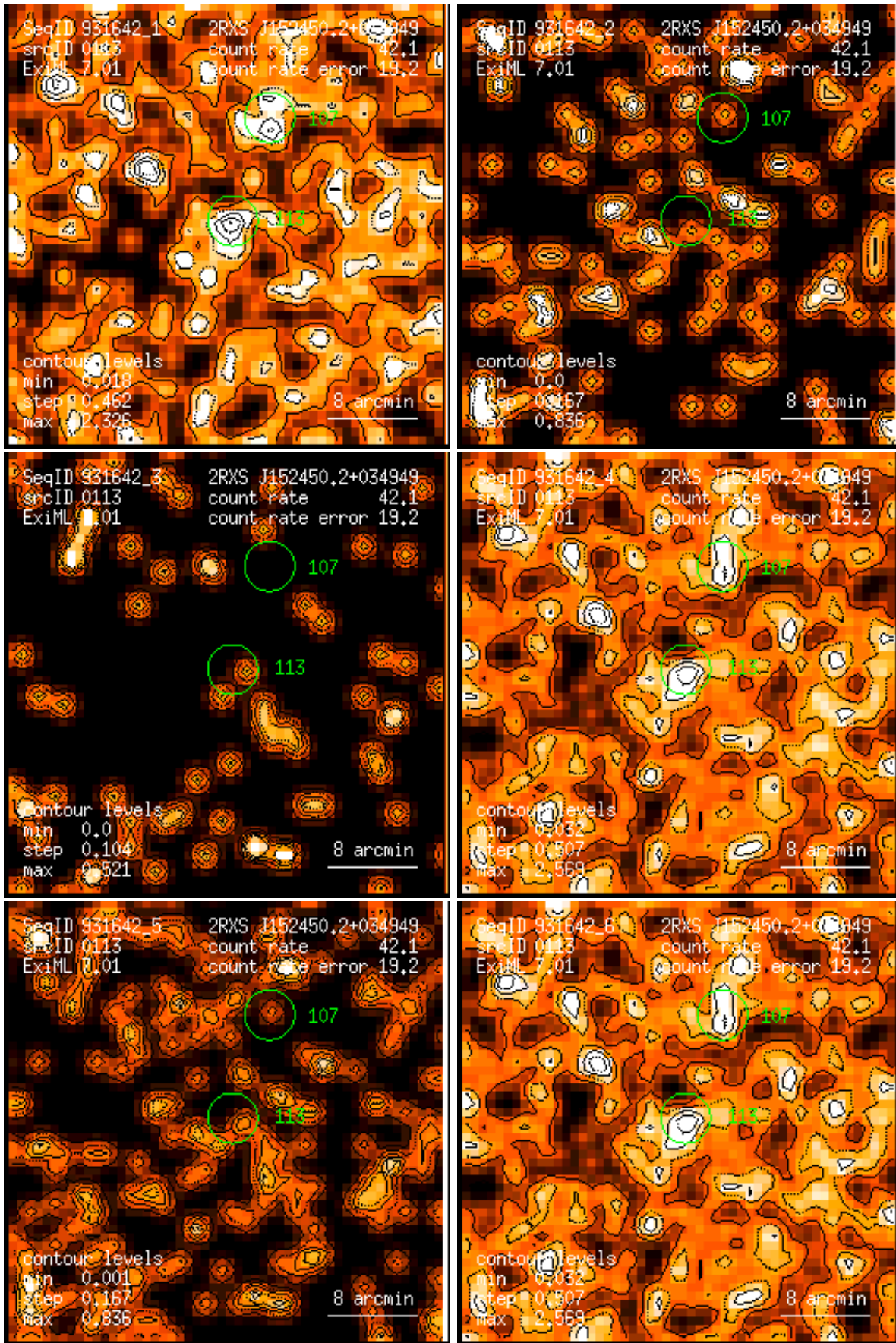
Figure 113: RASS 931642: detection 0113: band rate images, Gaussian filter: (1) PSPC channels 11 – 41, (2) 52 – 90, (3) 91 – 201, (4) 11 – 235, (5) 52 – 201, (6) 11 – 201. Broad band rates in counts/ks. Band rate contour levels in counts/ks/arcmin 2 .
