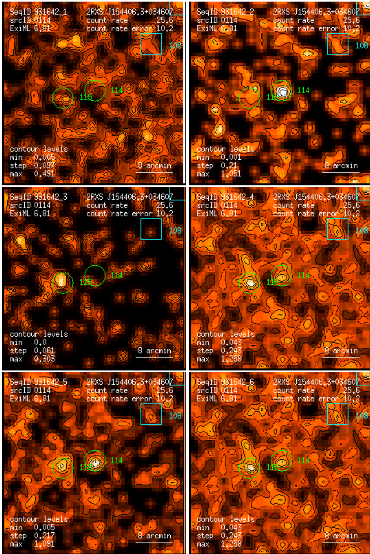
Figure 114: RASS 931642: detection 0114: band rate images, Gaussian filter: (1) PSPC channels 11 – 41, (2) 52 – 90, (3) 91 – 201, (4) 11 – 235, (5) 52 – 201, (6) 11 – 201. Broad band rates in counts/ks. Band rate contour levels in counts/ks/arcmin 2 .
