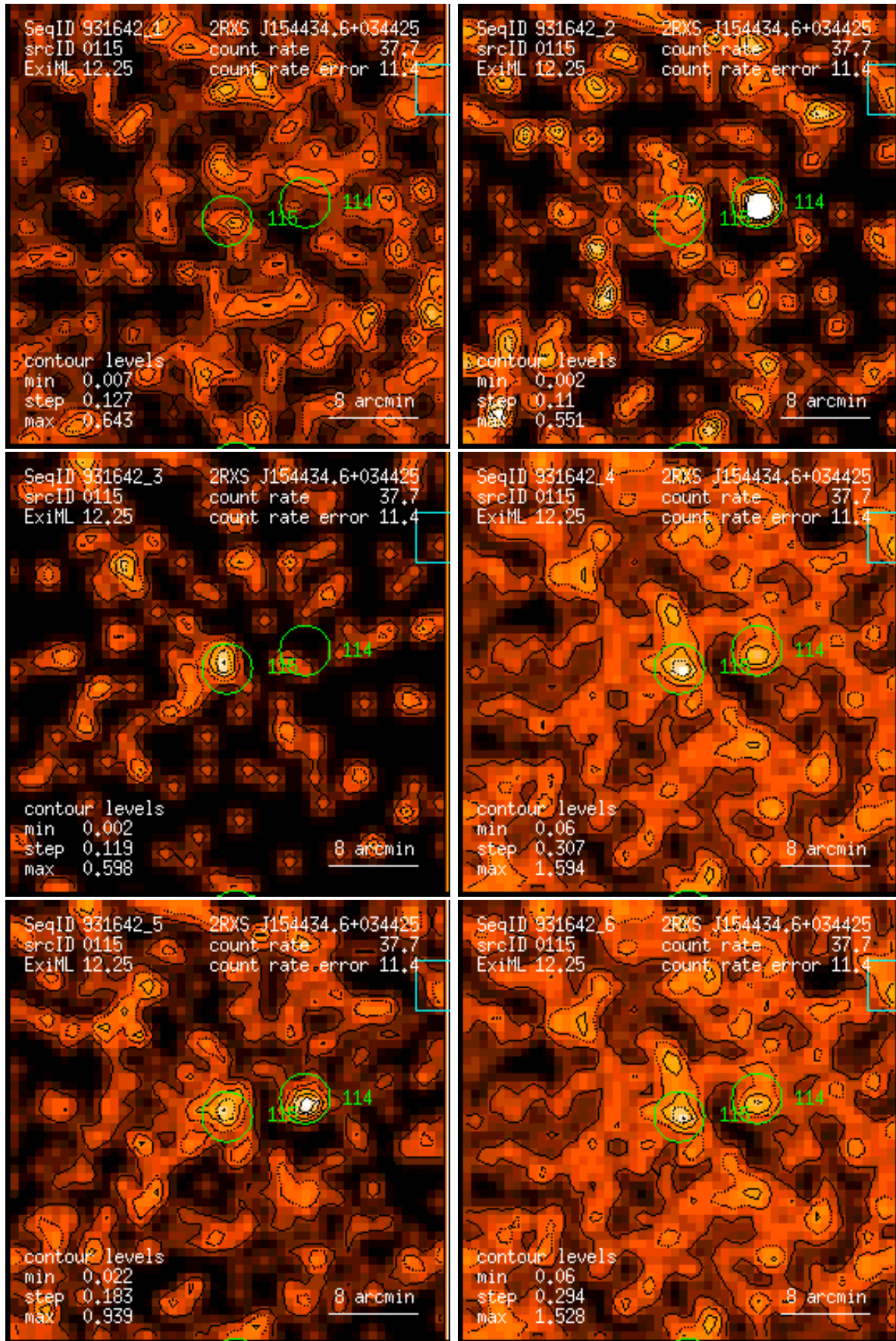
Figure 115: RASS 931642: detection 0115: band rate images, Gaussian filter: (1) PSPC channels 11 – 41, (2) 52 – 90, (3) 91 – 201, (4) 11 – 235, (5) 52 – 201, (6) 11 – 201. Broad band rates in counts/ks. Band rate contour levels in counts/ks/arcmin 2 .
