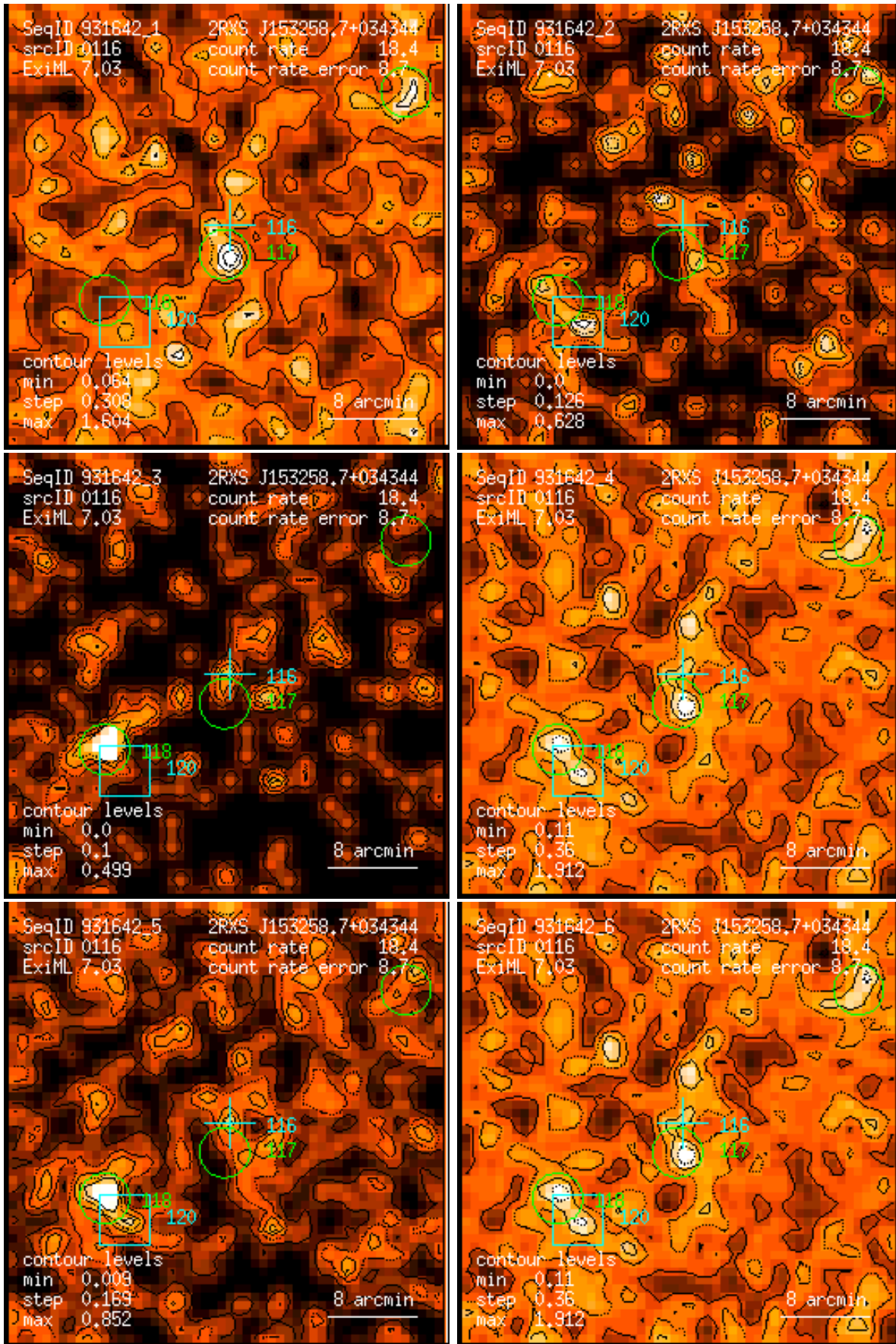
Figure 116: RASS 931642: detection 0116: band rate images, Gaussian filter: (1) PSPC channels 11 – 41, (2) 52 – 90, (3) 91 – 201, (4) 11 – 235, (5) 52 – 201, (6) 11 – 201. Broad band rates in counts/ks. Band rate contour levels in counts/ks/arcmin 2 .
