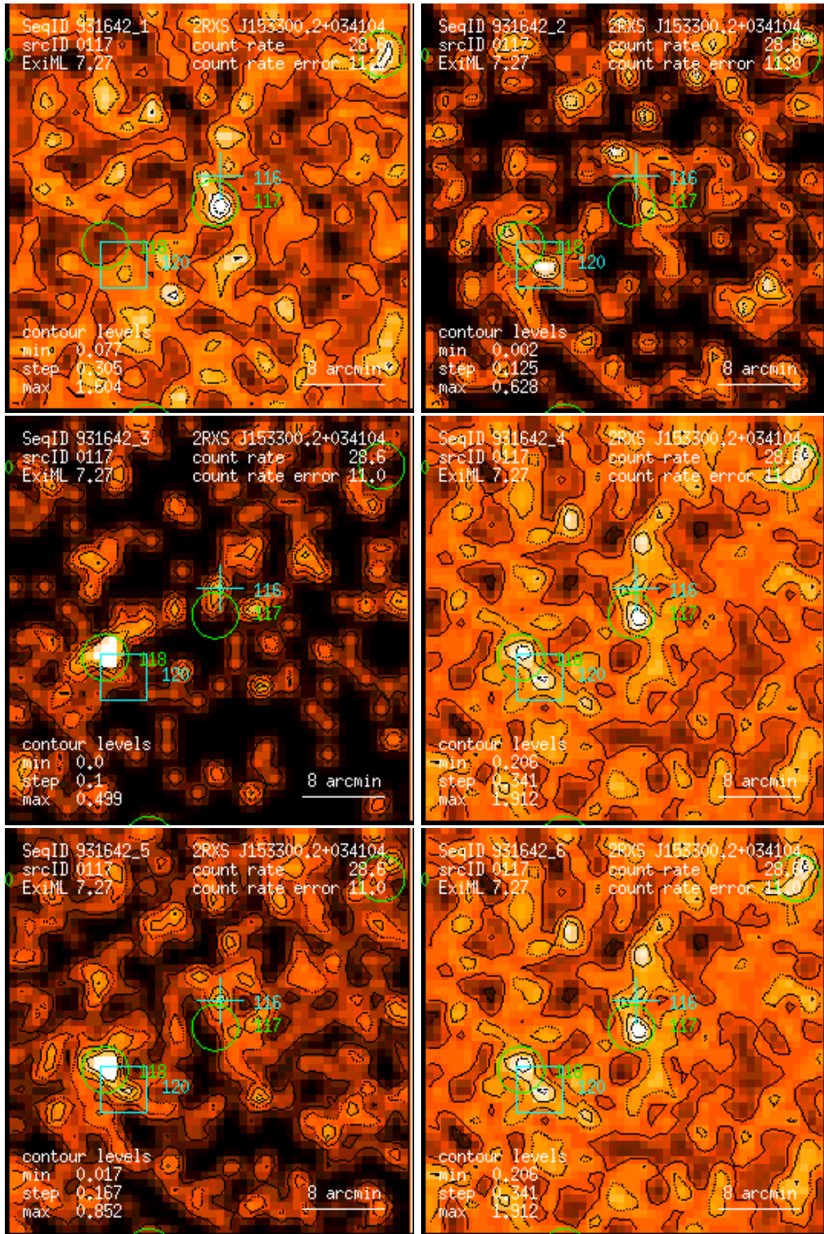
Figure 117: RASS 931642: detection 0117: band rate images, Gaussian filter: (1) PSPC channels 11 – 41, (2) 52 – 90, (3) 91 – 201, (4) 11 – 235, (5) 52 – 201, (6) 11 – 201. Broad band rates in counts/ks. Band rate contour levels in counts/ks/arcmin 2 .
