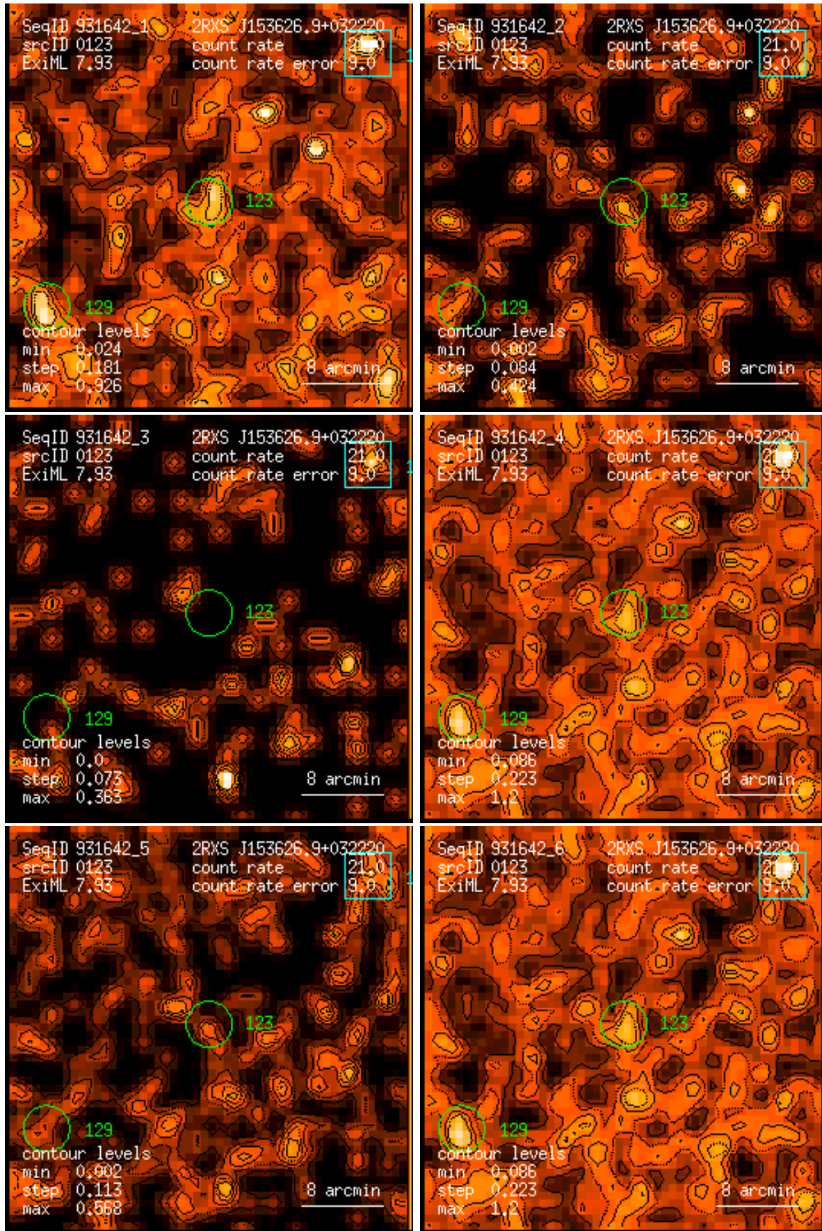
Figure 123: RASS 931642: detection 0123: band rate images, Gaussian filter: (1) PSPC channels 11 – 41, (2) 52 – 90, (3) 91 – 201, (4) 11 – 235, (5) 52 – 201, (6) 11 – 201. Broad band rates in counts/ks. Band rate contour levels in counts/ks/arcmin 2 .
