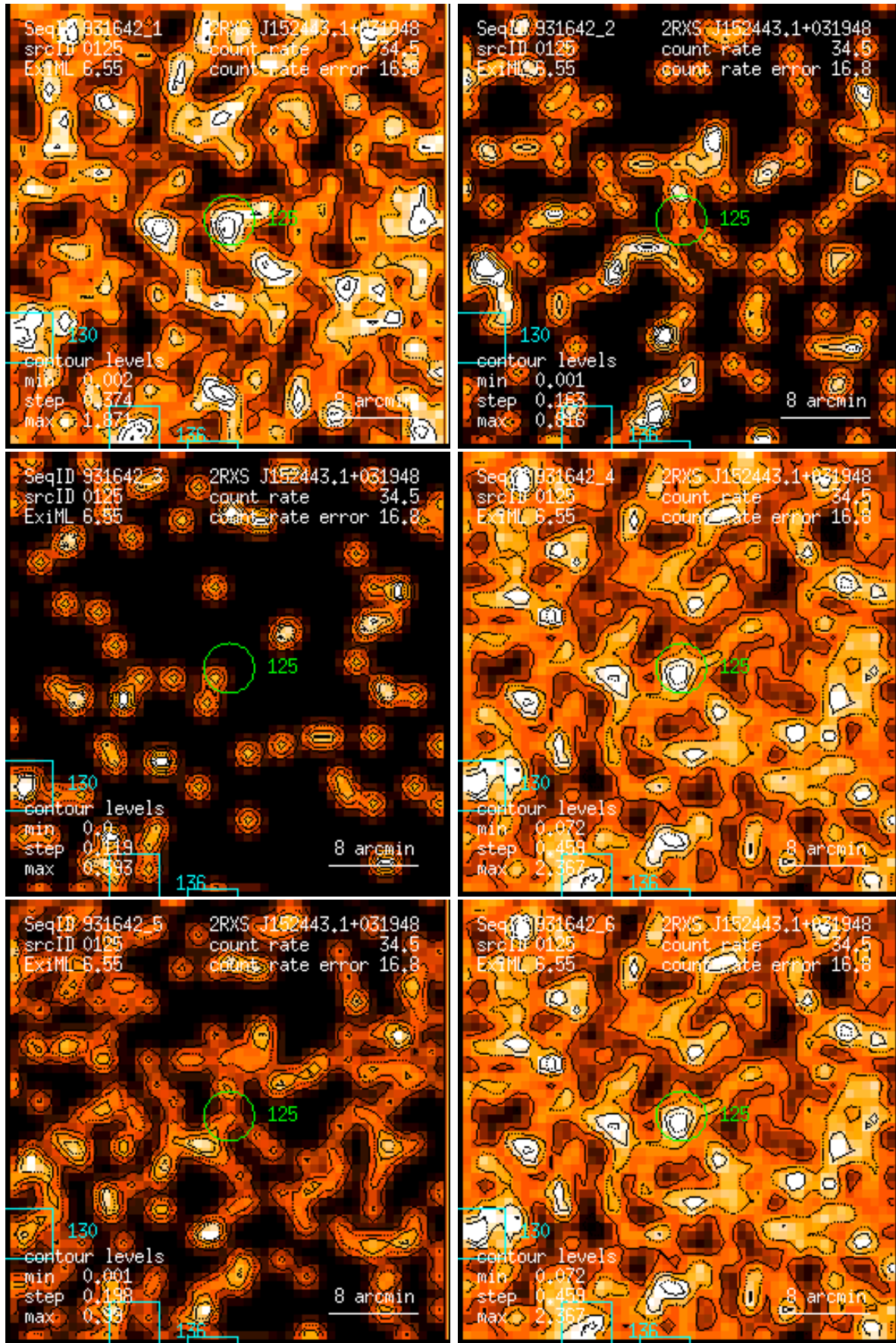
Figure 125: RASS 931642: detection 0125: band rate images, Gaussian filter: (1) PSPC channels 11 – 41, (2) 52 – 90, (3) 91 – 201, (4) 11 – 235, (5) 52 – 201, (6) 11 – 201. Broad band rates in counts/ks. Band rate contour levels in counts/ks/arcmin 2 .
