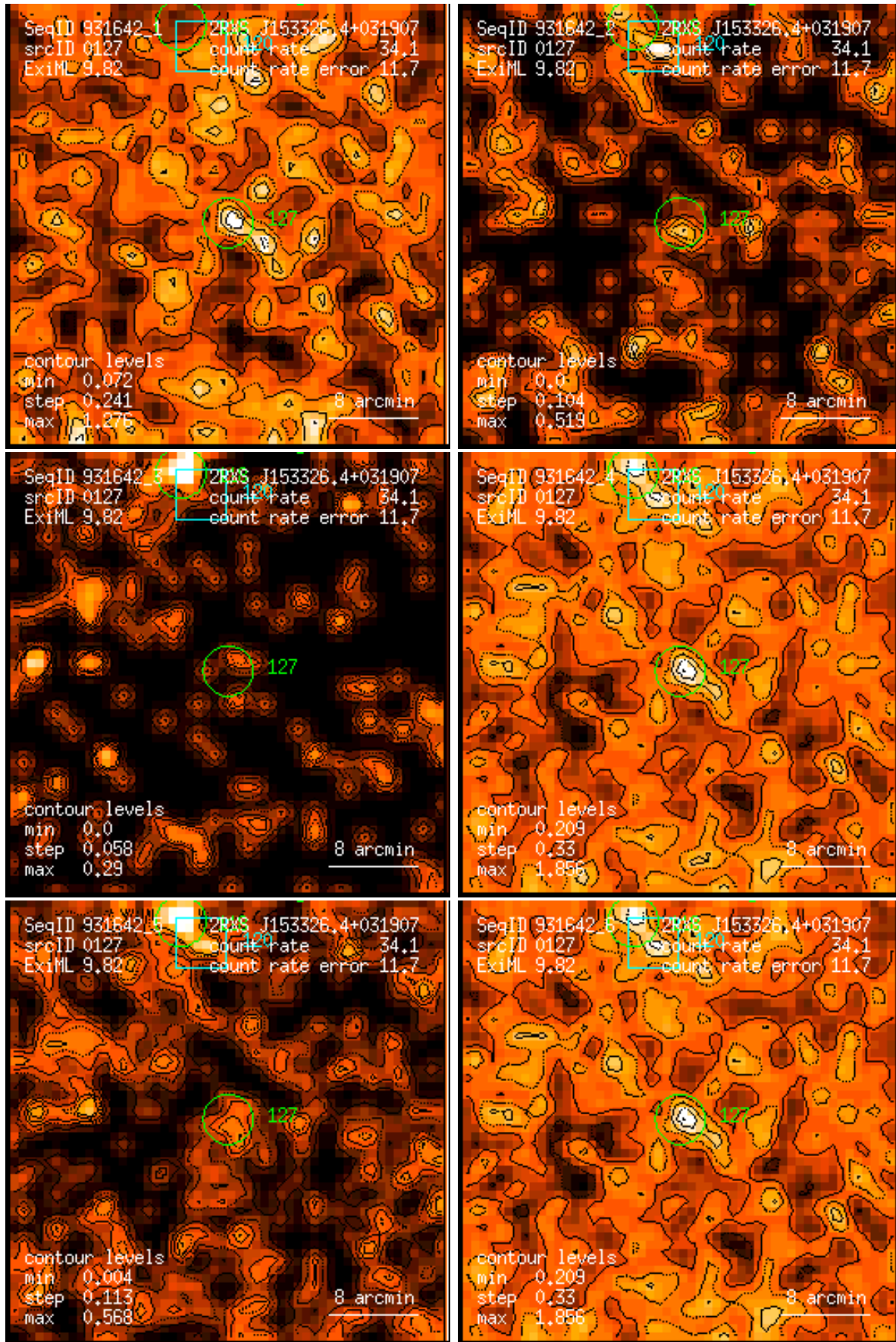
Figure 127: RASS 931642: detection 0127: band rate images, Gaussian filter: (1) PSPC channels 11 – 41, (2) 52 – 90, (3) 91 – 201, (4) 11 – 235, (5) 52 – 201, (6) 11 – 201. Broad band rates in counts/ks. Band rate contour levels in counts/ks/arcmin 2 .
