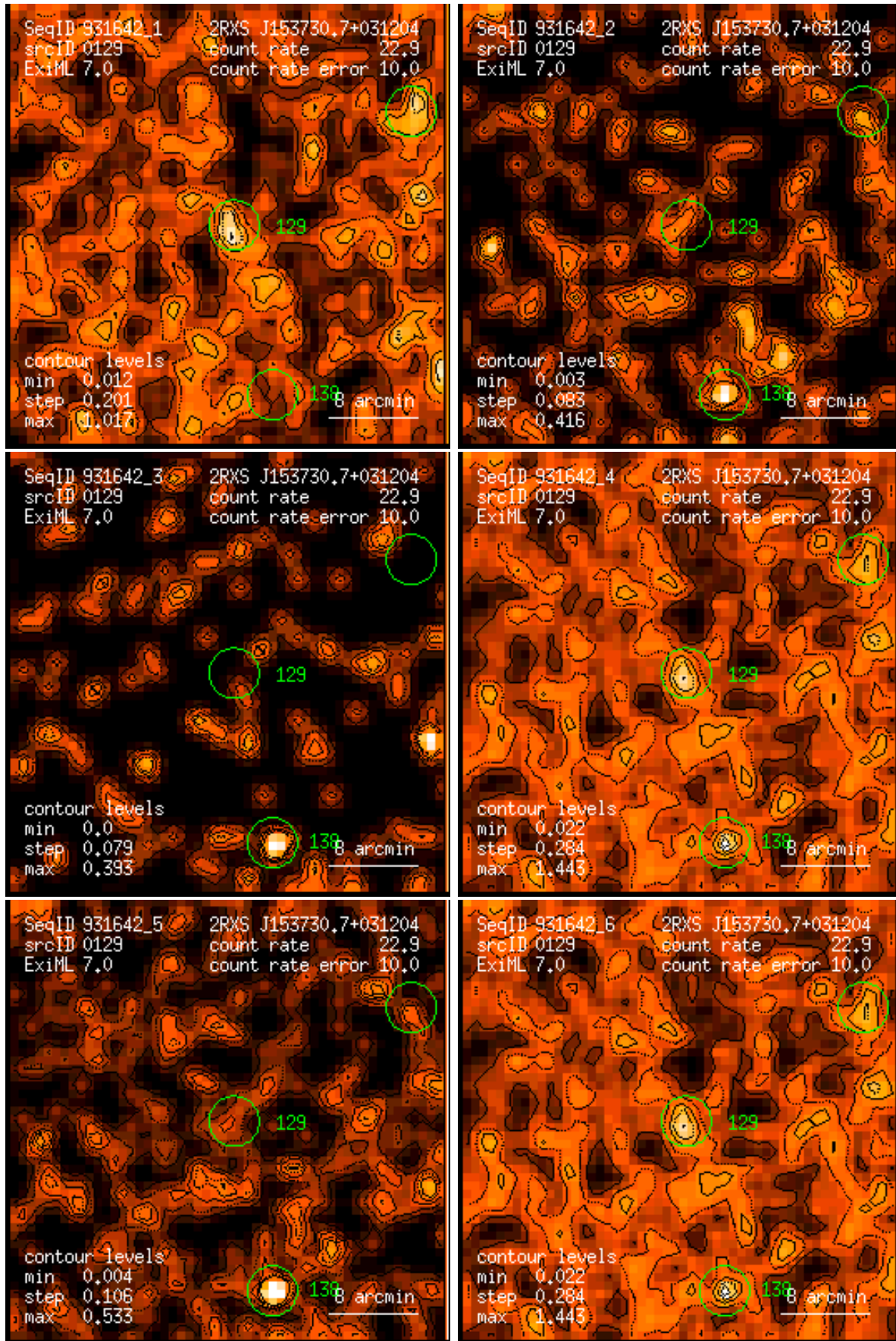
Figure 129: RASS 931642: detection 0129: band rate images, Gaussian filter: (1) PSPC channels 11 – 41, (2) 52 – 90, (3) 91 – 201, (4) 11 – 235, (5) 52 – 201, (6) 11 – 201. Broad band rates in counts/ks. Band rate contour levels in counts/ks/arcmin 2 .
