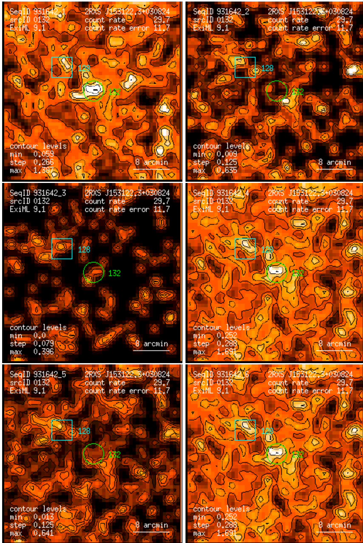
Figure 132: RASS 931642: detection 0132: band rate images, Gaussian filter: (1) PSPC channels 11 – 41, (2) 52 – 90, (3) 91 – 201, (4) 11 – 235, (5) 52 – 201, (6) 11 – 201. Broad band rates in counts/ks. Band rate contour levels in counts/ks/arcmin 2 .
