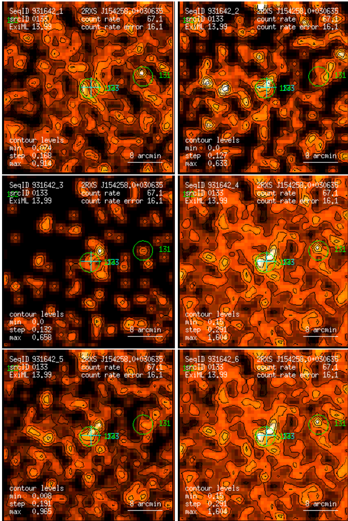
Figure 133: RASS 931642: detection 0133: band rate images, Gaussian filter: (1) PSPC channels 11 – 41, (2) 52 – 90, (3) 91 – 201, (4) 11 – 235, (5) 52 – 201, (6) 11 – 201. Broad band rates in counts/ks. Band rate contour levels in counts/ks/arcmin 2 .
