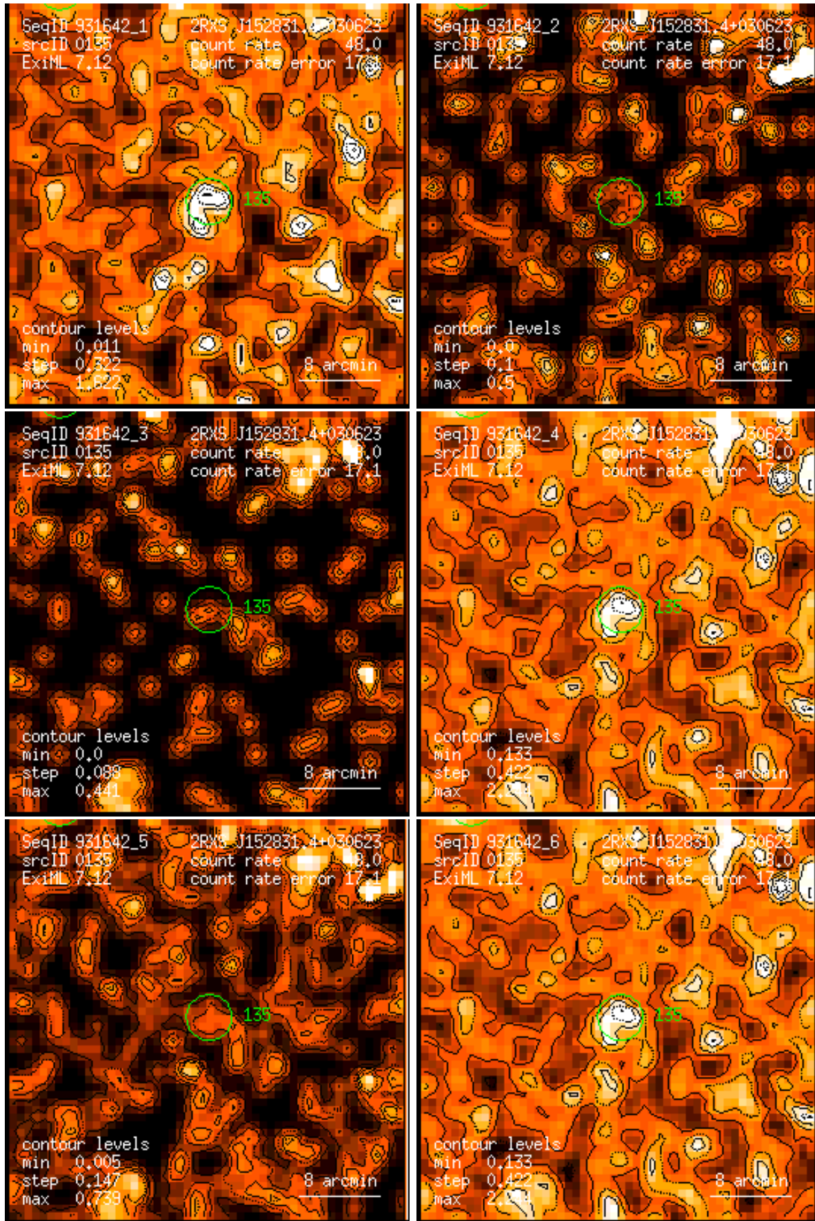
Figure 135: RASS 931642: detection 0135: band rate images, Gaussian filter: (1) PSPC channels 11 – 41, (2) 52 – 90, (3) 91 – 201, (4) 11 – 235, (5) 52 – 201, (6) 11 – 201. Broad band rates in counts/ks. Band rate contour levels in counts/ks/arcmin 2 .
