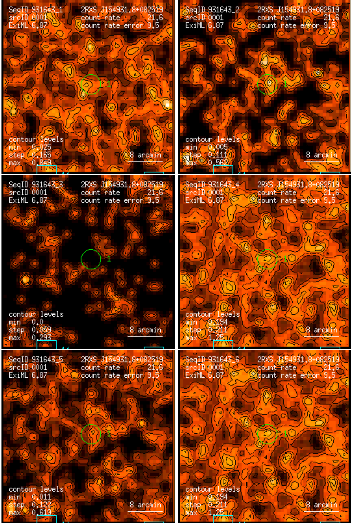
Figure 1: RASS 931643: detection 0001: band rate images, Gaussian filter: (1) PSPC channels 11 – 41, (2) 52 – 90, (3) 91 – 201, (4) 11 – 235, (5) 52 – 201, (6) 11 – 201. Broad band rates in counts/ks. Band rate contour levels in counts/ks/arcmin 2 .
