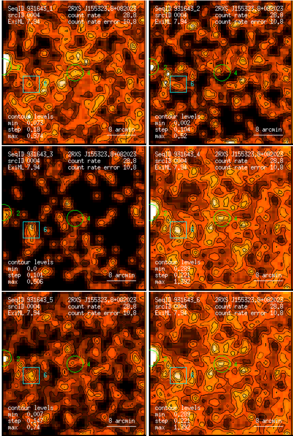
Figure 4: RASS 931643: detection 0004: band rate images, Gaussian filter: (1) PSPC channels 11 – 41, (2) 52 – 90, (3) 91 – 201, (4) 11 – 235, (5) 52 – 201, (6) 11 – 201. Broad band rates in counts/ks. Band rate contour levels in counts/ks/arcmin 2 .
