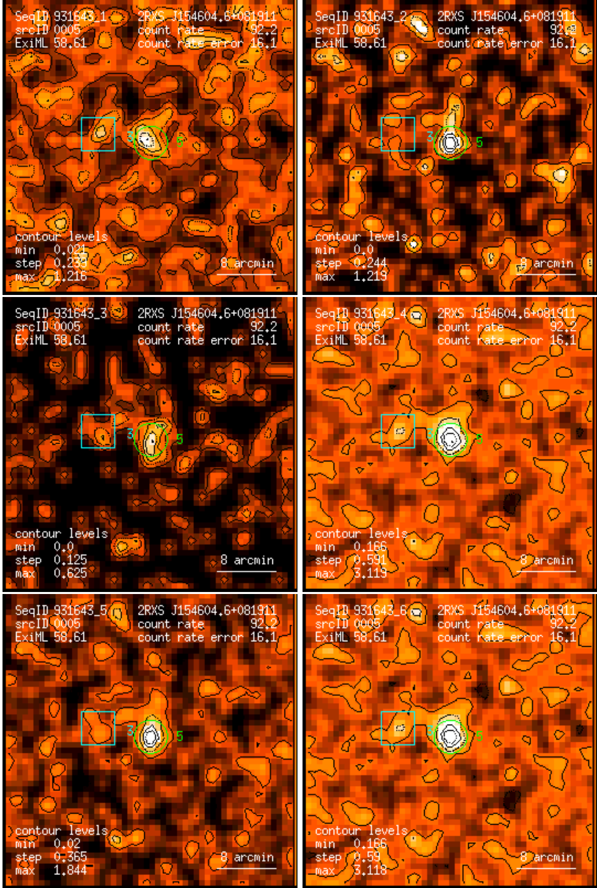
Figure 5: RASS 931643: detection 0005: band rate images, Gaussian filter: (1) PSPC channels 11 – 41, (2) 52 – 90, (3) 91 – 201, (4) 11 – 235, (5) 52 – 201, (6) 11 – 201. Broad band rates in counts/ks. Band rate contour levels in counts/ks/arcmin 2 .
