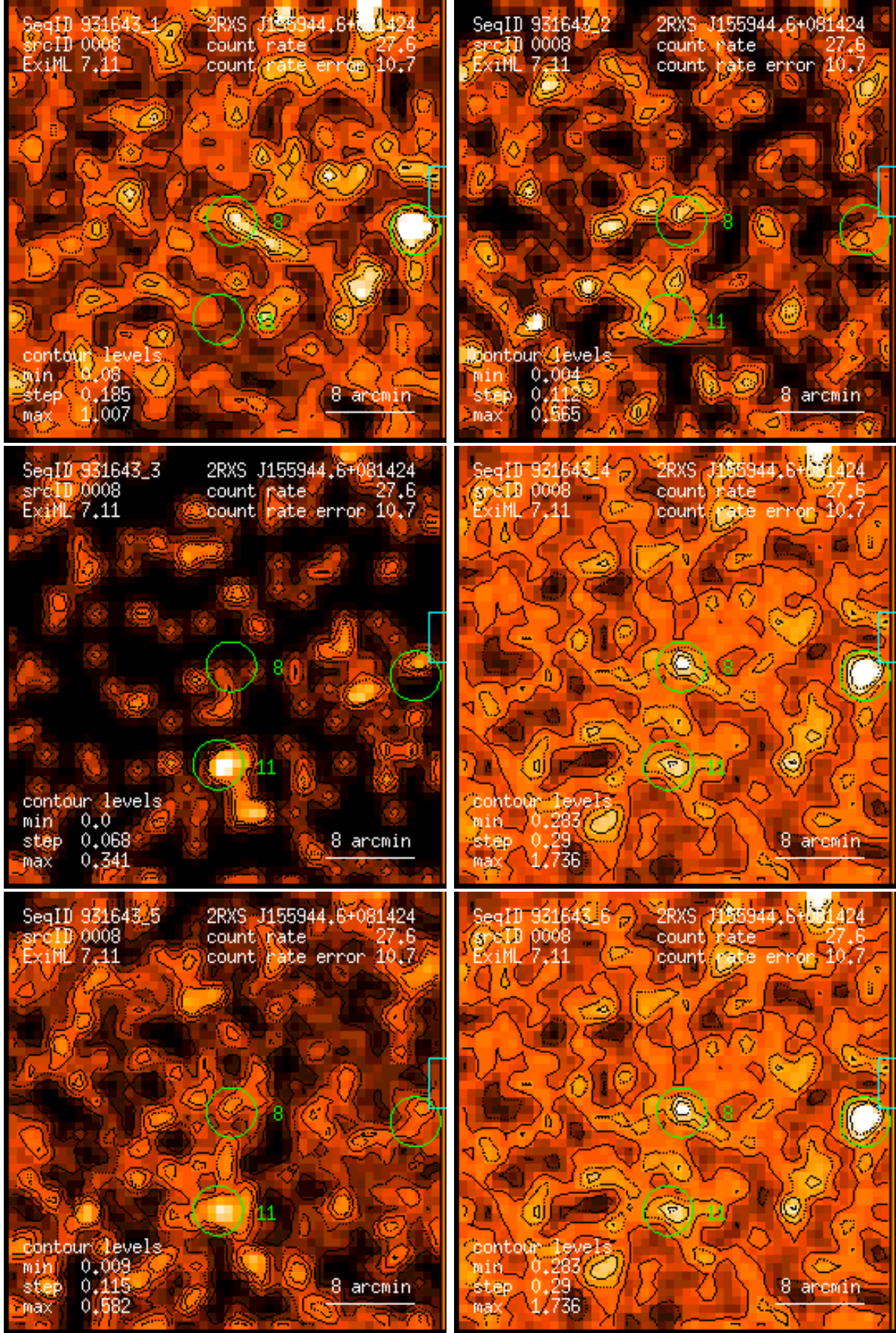
Figure 8: RASS 931643: detection 0008: band rate images, Gaussian filter: (1) PSPC channels 11 – 41, (2) 52 – 90, (3) 91 – 201, (4) 11 – 235, (5) 52 – 201, (6) 11 – 201. Broad band rates in counts/ks. Band rate contour levels in counts/ks/arcmin 2 .
