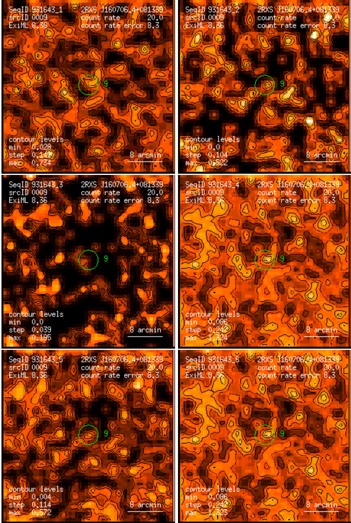
Figure 9: RASS 931643: detection 0009: band rate images, Gaussian filter: (1) PSPC channels 11 – 41, (2) 52 – 90, (3) 91 – 201, (4) 11 – 235, (5) 52 – 201, (6) 11 – 201. Broad band rates in counts/ks. Band rate contour levels in counts/ks/arcmin 2 .
