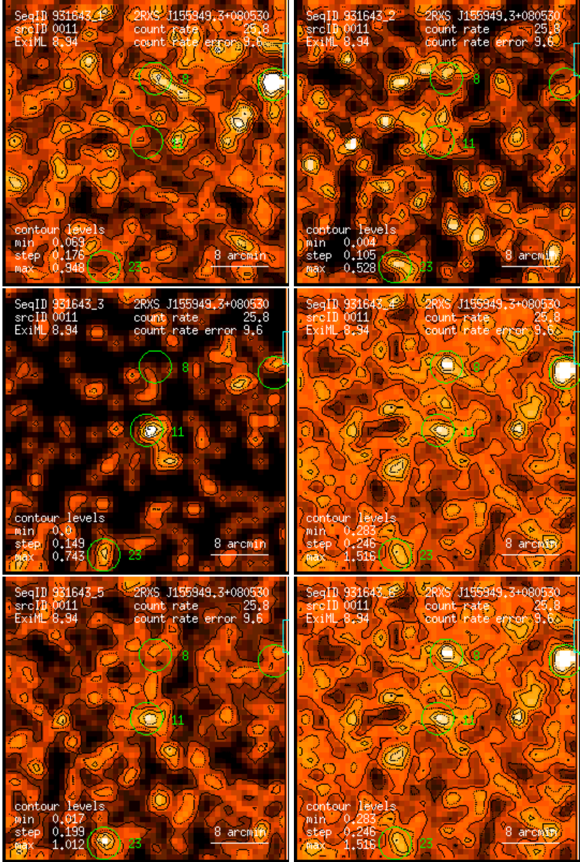
Figure 11: RASS 931643: detection 0011: band rate images, Gaussian filter: (1) PSPC channels 11 – 41, (2) 52 – 90, (3) 91 – 201, (4) 11 – 235, (5) 52 – 201, (6) 11 – 201. Broad band rates in counts/ks. Band rate contour levels in counts/ks/arcmin 2 .
