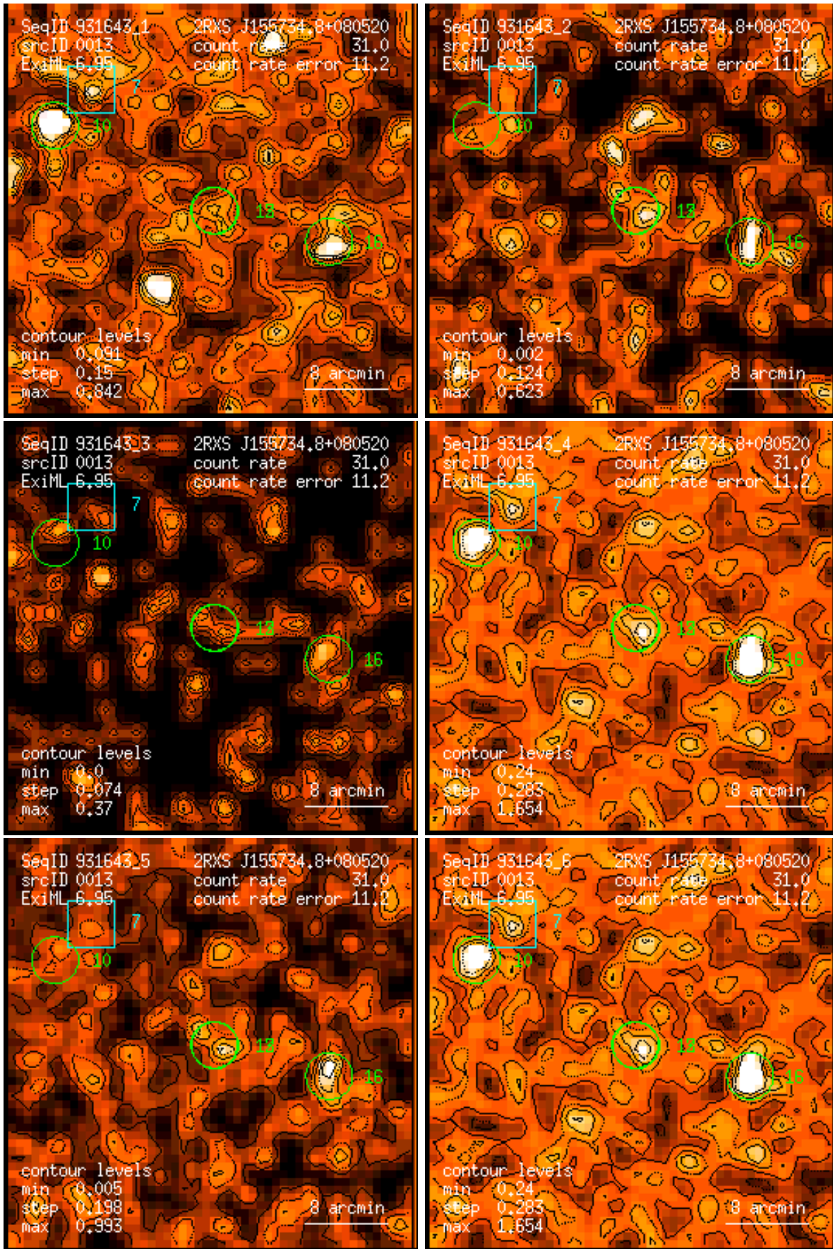
Figure 13: RASS 931643: detection 0013: band rate images, Gaussian filter: (1) PSPC channels 11 – 41, (2) 52 – 90, (3) 91 – 201, (4) 11 – 235, (5) 52 – 201, (6) 11 – 201. Broad band rates in counts/ks. Band rate contour levels in counts/ks/arcmin 2 .
