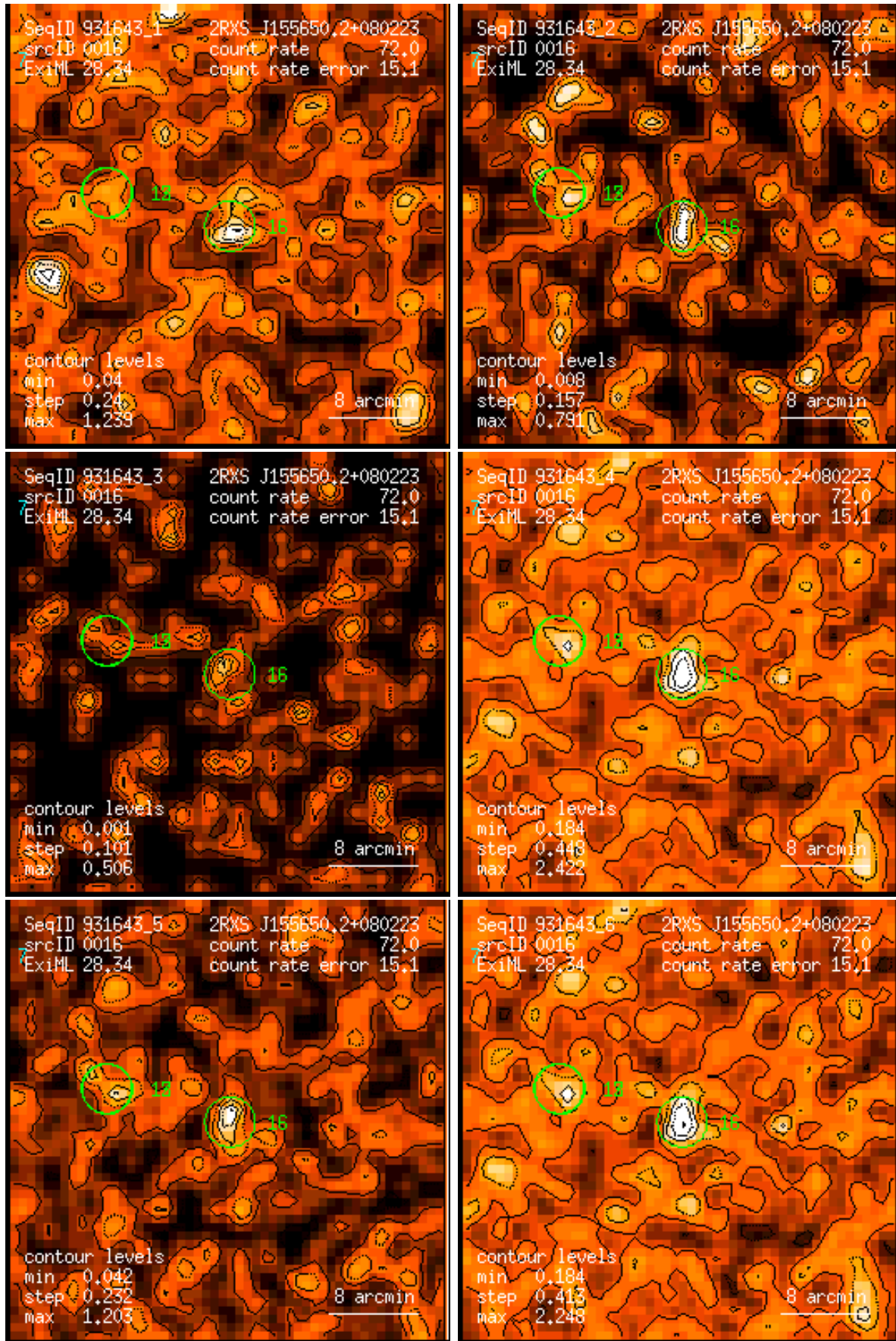
Figure 16: RASS 931643: detection 0016: band rate images, Gaussian filter: (1) PSPC channels 11 – 41, (2) 52 – 90, (3) 91 – 201, (4) 11 – 235, (5) 52 – 201, (6) 11 – 201. Broad band rates in counts/ks. Band rate contour levels in counts/ks/arcmin 2 .
