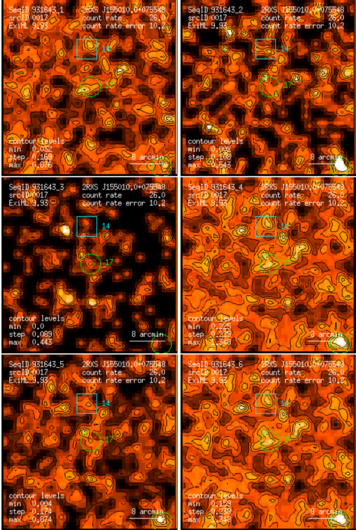
Figure 17: RASS 931643: detection 0017: band rate images, Gaussian filter: (1) PSPC channels 11 – 41, (2) 52 – 90, (3) 91 – 201, (4) 11 – 235, (5) 52 – 201, (6) 11 – 201. Broad band rates in counts/ks. Band rate contour levels in counts/ks/arcmin 2 .
