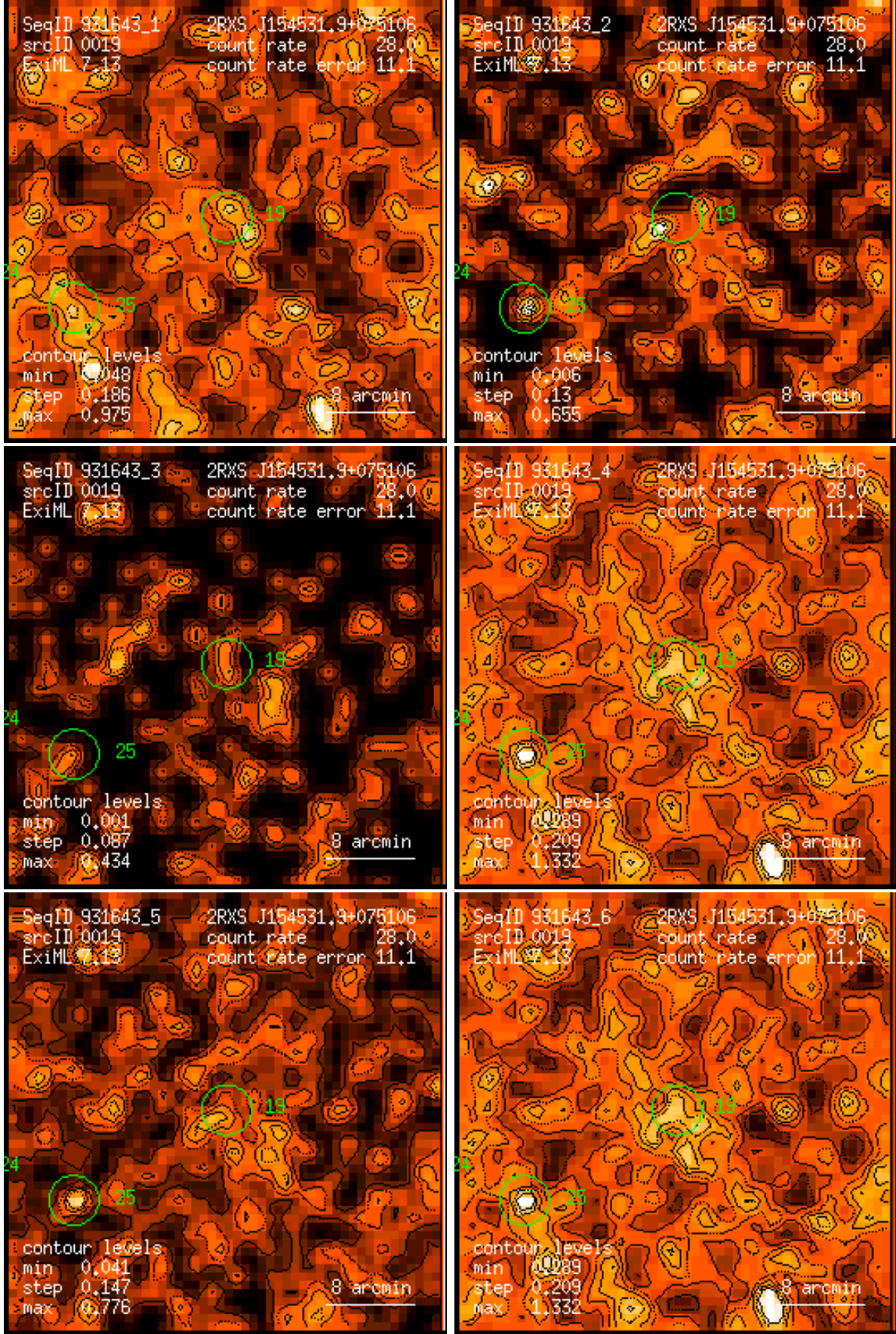
Figure 19: RASS 931643: detection 0019: band rate images, Gaussian filter: (1) PSPC channels 11 – 41, (2) 52 – 90, (3) 91 – 201, (4) 11 – 235, (5) 52 – 201, (6) 11 – 201. Broad band rates in counts/ks. Band rate contour levels in counts/ks/arcmin 2 .
